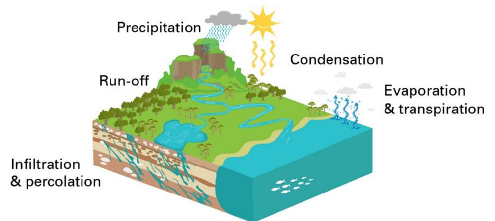
Natural water cycle
