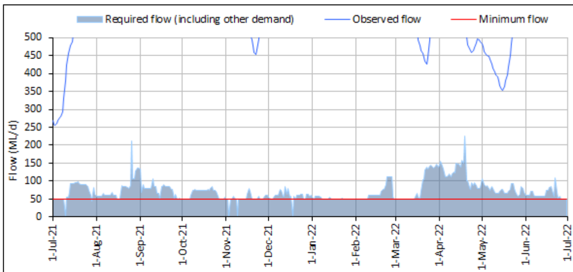
Figure 55: Billabong Creek at Darlot flow and target
