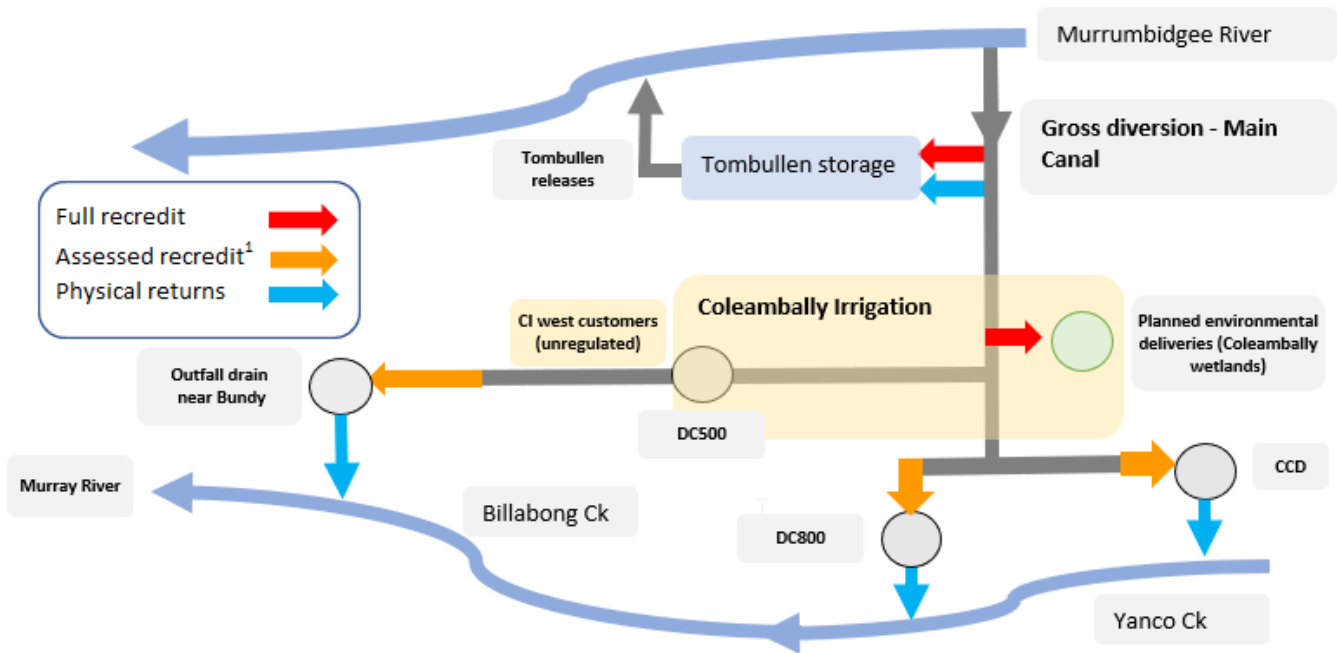
Figure 51: Conceptual diagram for Coleambally Irrigation re-credits
