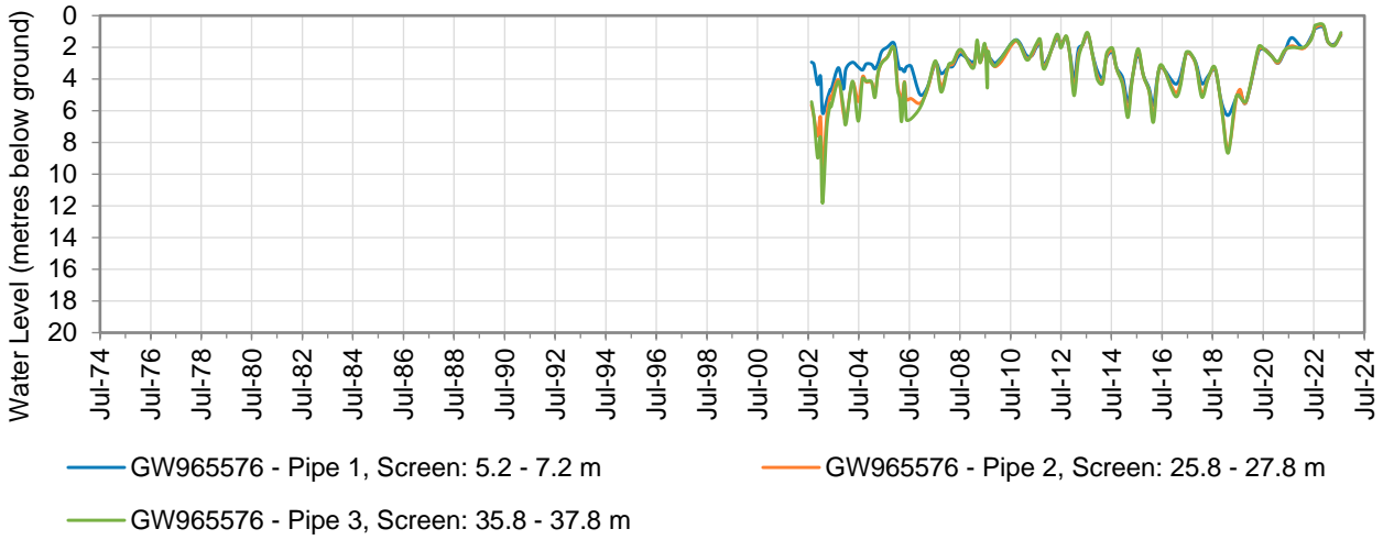
Figure 8: Hydrograph of monitoring bore GW965576
