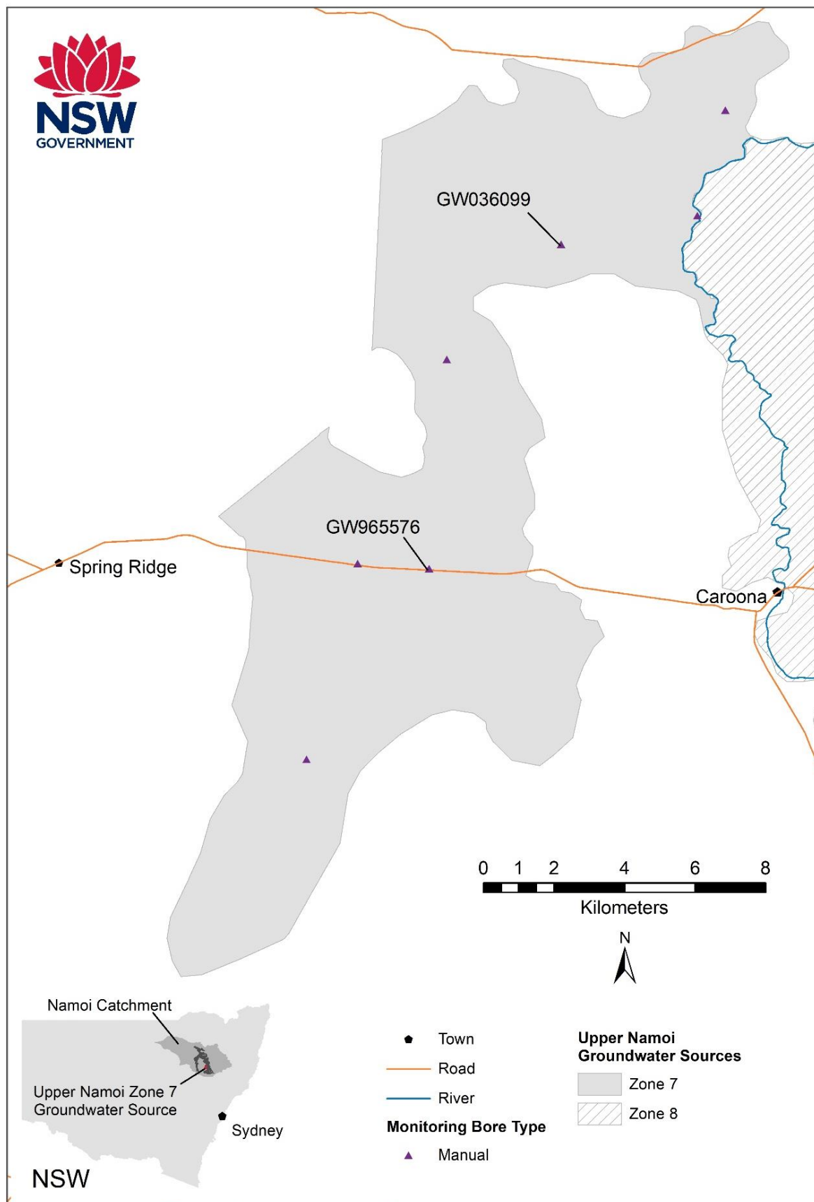
Figure 6: Upper Namoi Zone 7 Groundwater Source monitoring bore sites
