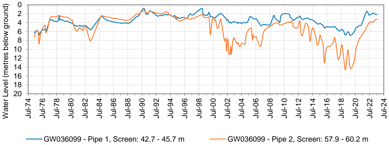
Figure 7: Hydrograph for monitoring bore GW036099
