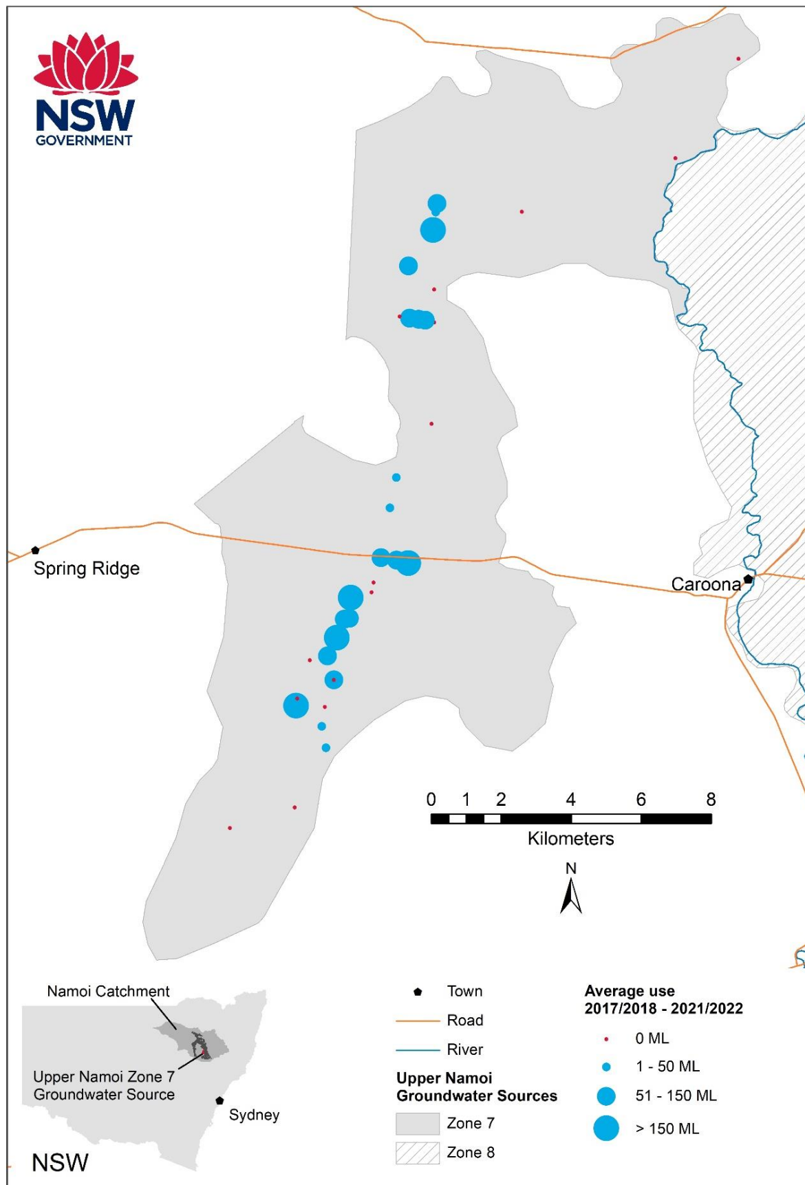
Figure 5: Upper Namoi Zone 7 Groundwater Source water supply bores and distribution of extraction
