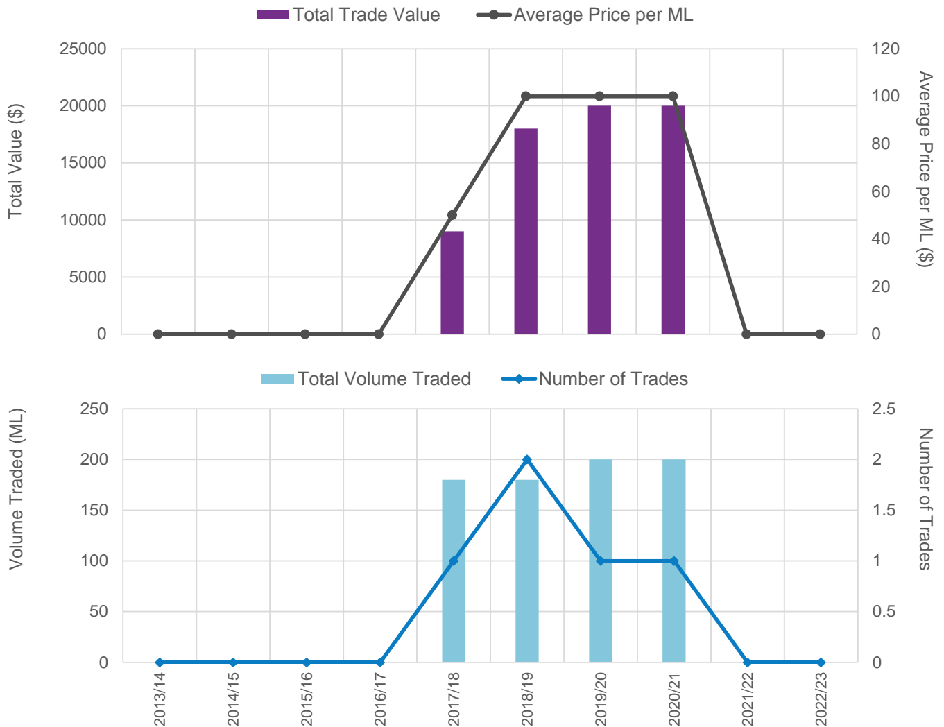
Figure 3: Upper Namoi Zone 7 Groundwater Source temporary trade statistics
