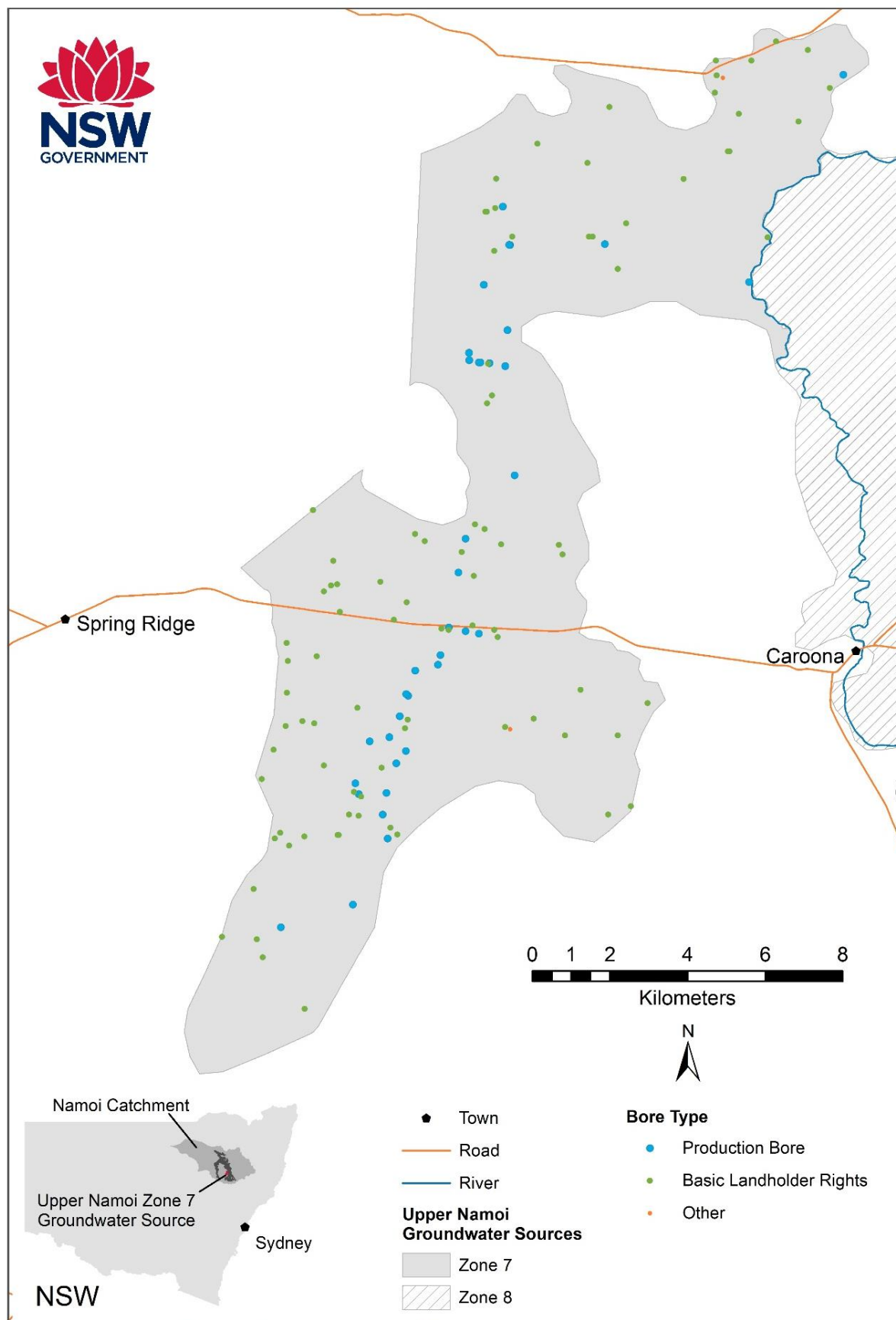
Figure 4: Upper Namoi Zone 7 Groundwater Source registered bores
