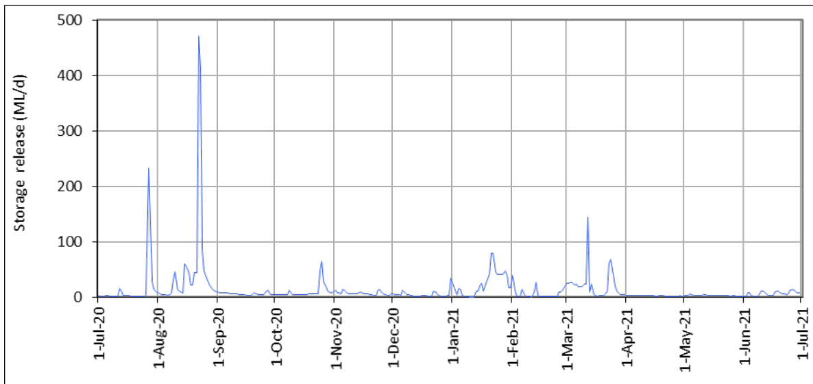
Figure 57: Carcoar Dam storage releases
