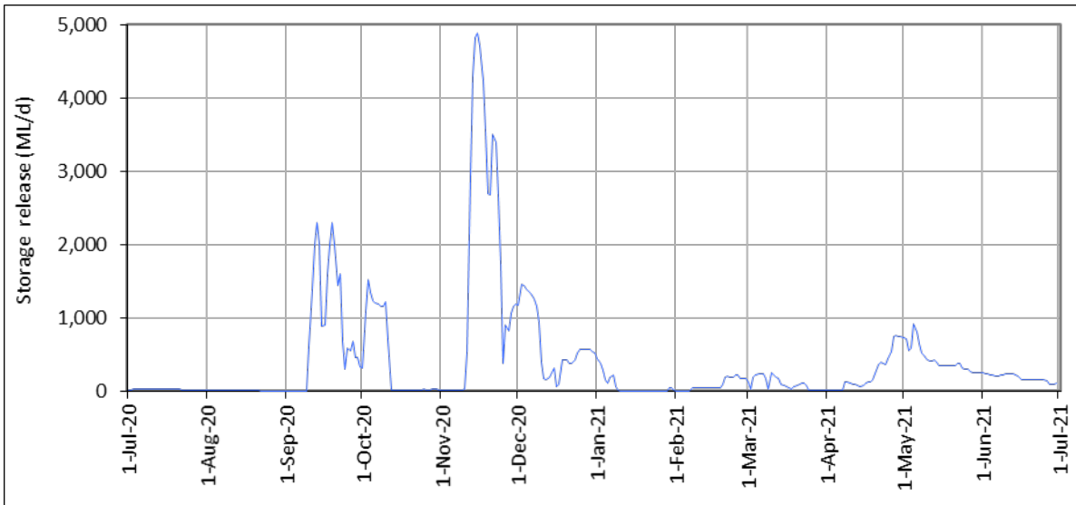
Figure 59: Lake Brewster storage release
