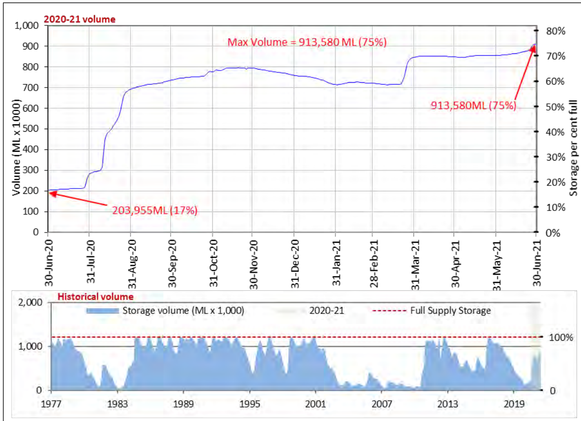
Figure 12: Wyangala Dam storage volume and per cent full for 2020–21
