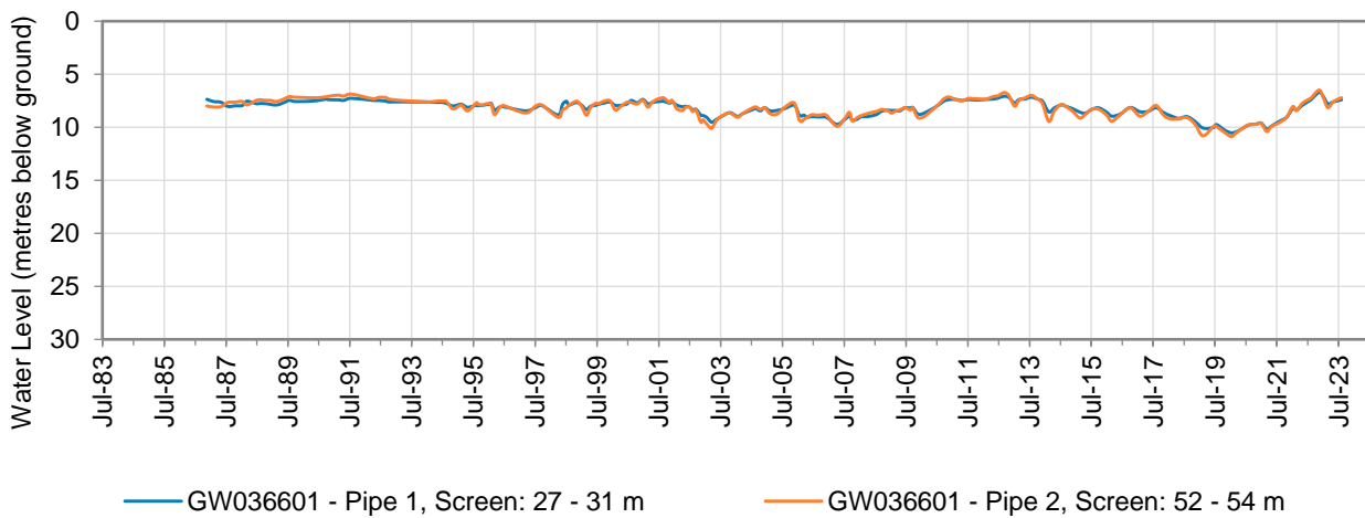
Figure 9: Hydrograph of monitoring bore GW036601
