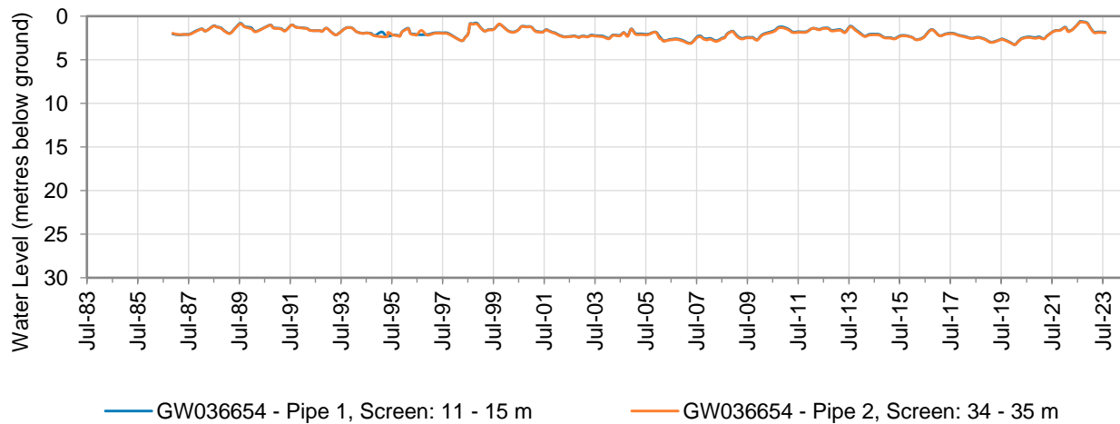
Figure 10: Hydrograph of monitoring bore GW036654
