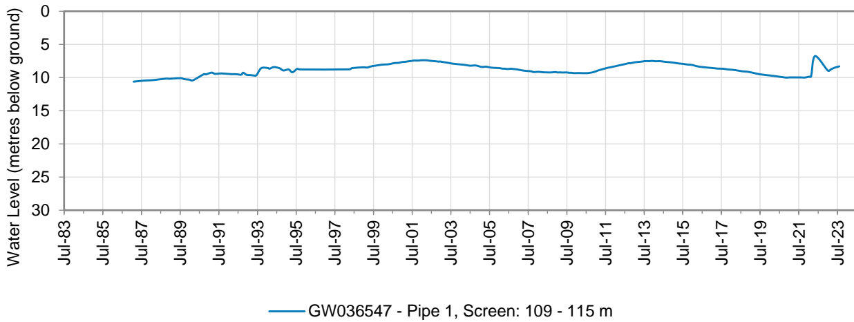
Figure 8: Hydrograph of monitoring bore GW036547
