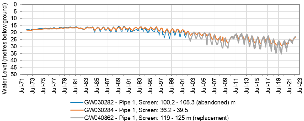
Figure 11: Hydrograph for monitoring bore GW040862
