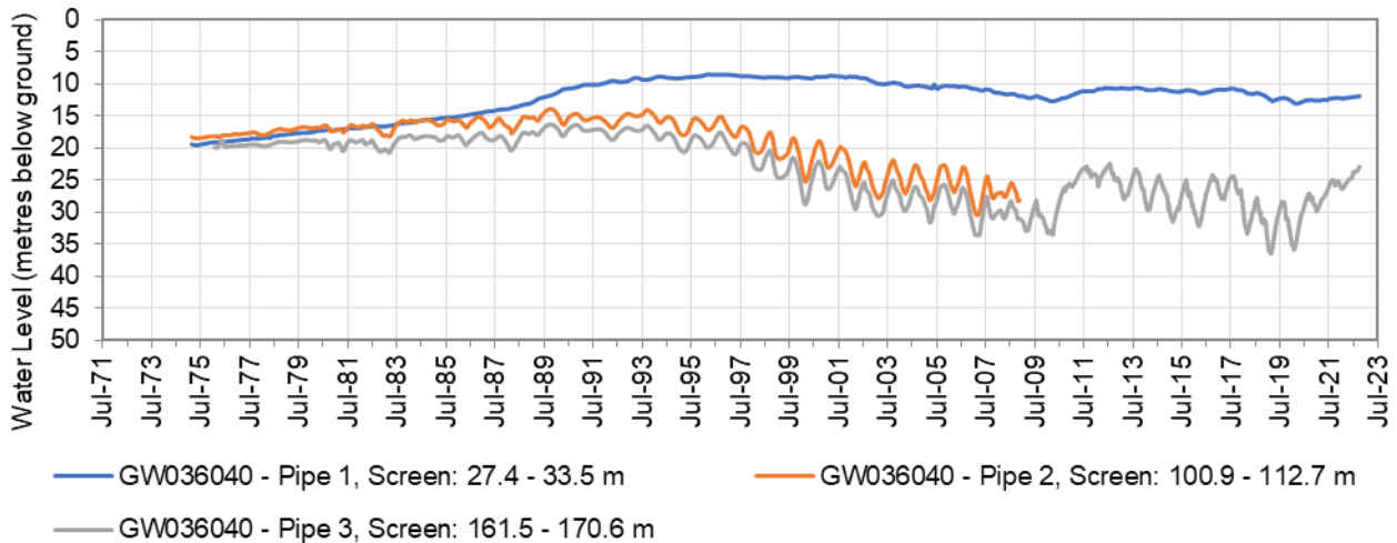
Figure 17: Hydrograph of monitoring bore GW036040
