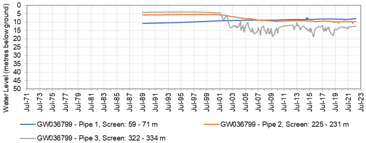
in Figure 10 to Figure 22: Hydrograph of monitoring bore GW036799
