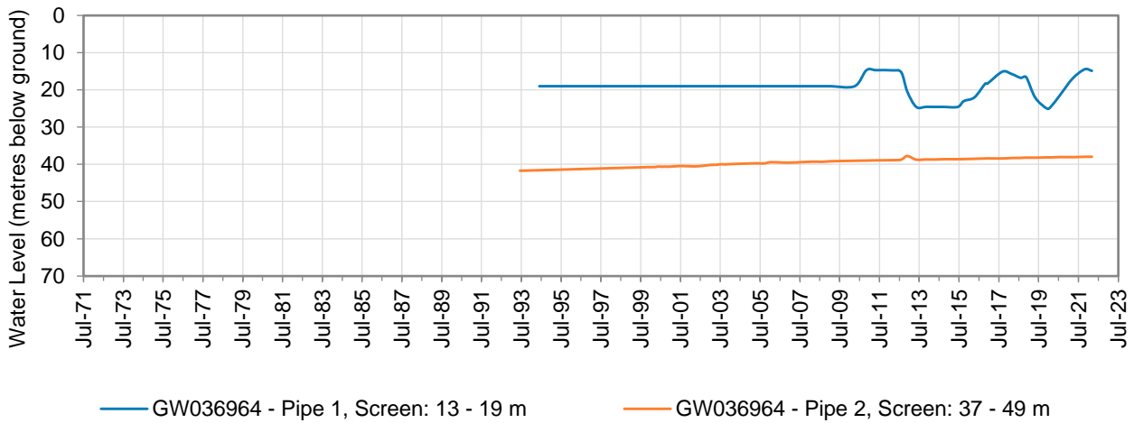
Figure 22: Hydrograph of monitoring bore GW036964 (Zone 5)
