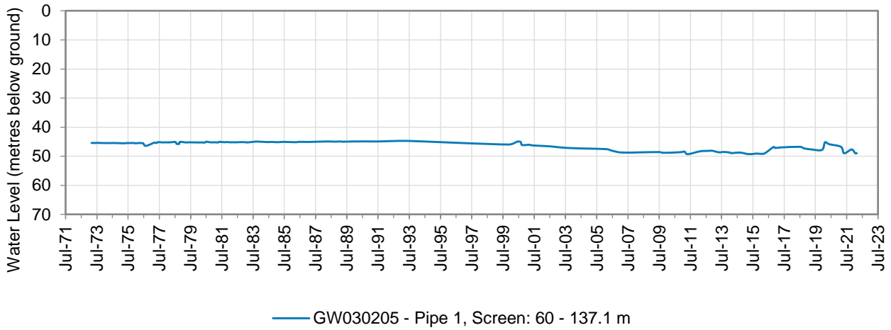
Figure 17: Hydrograph of monitoring bore GW030205 (Zone 4)
