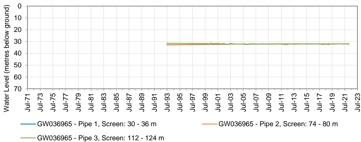
Figure 23: Hydrograph of monitoring bore GW036965 (Zone 5)
