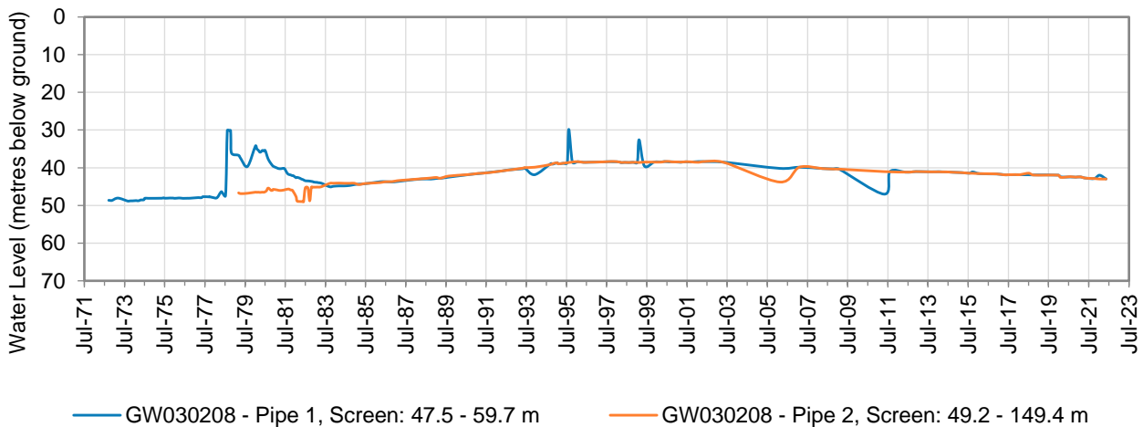
Figure 13: Hydrograph of monitoring bore GW030208 (Zone 4)
