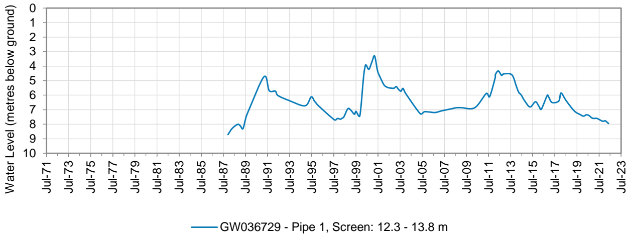
Figure 12: Hydrograph of monitoring bore GW036729 (Zone 3)
