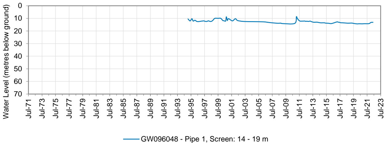
Figure 10: Hydrograph for monitoring bore GW096048 (Zone 3)
