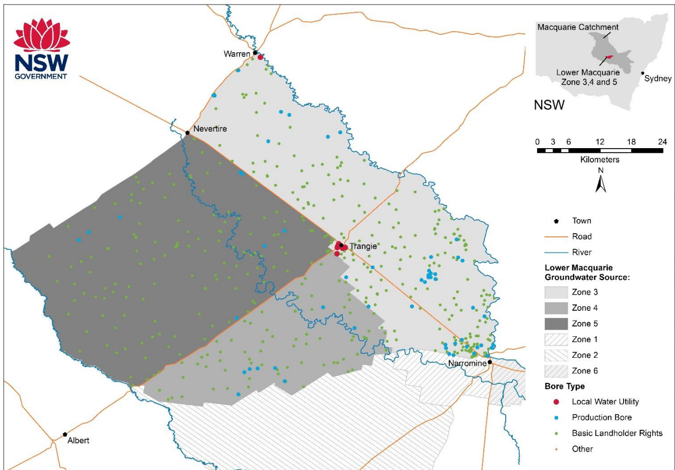
Figure 7: Lower Macquarie sandstone groundwater sources Zones 3, 4 and 5 registered bores
