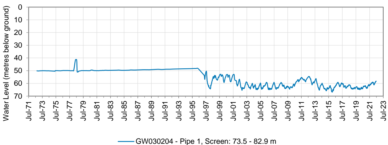
Figure 16: Hydrograph of monitoring bore GW030204 (Zone 4)
