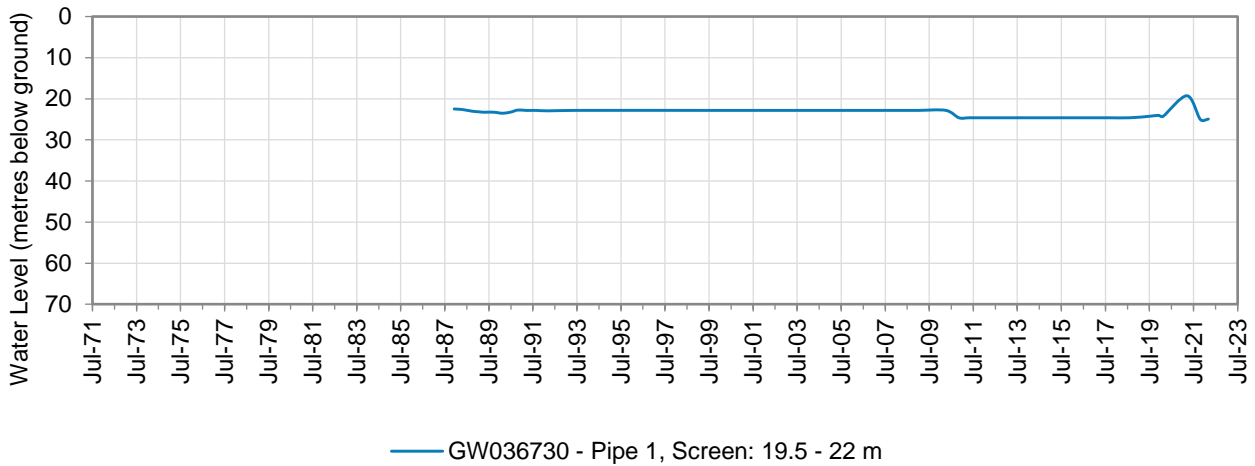
Figure 21: Hydrograph of monitoring bore GW036730 (Zone 5)
