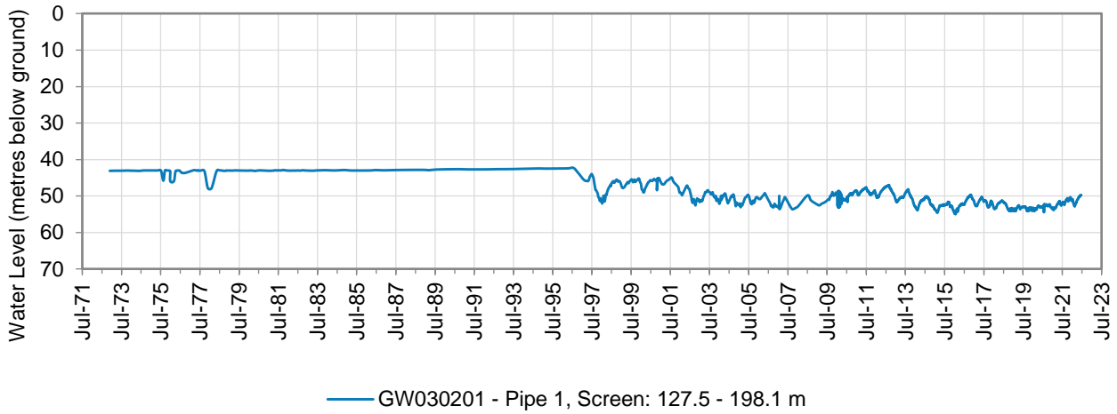
Figure 20: Hydrograph of monitoring bore GW030201 (Zone 4 / Zone 5 Boundary)
