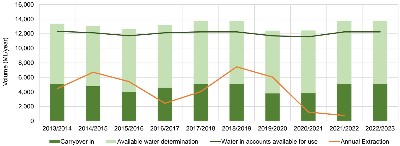
Figure 3: Account water availability and usage summary for Lower Macquarie Zone 4 Groundwater Source
