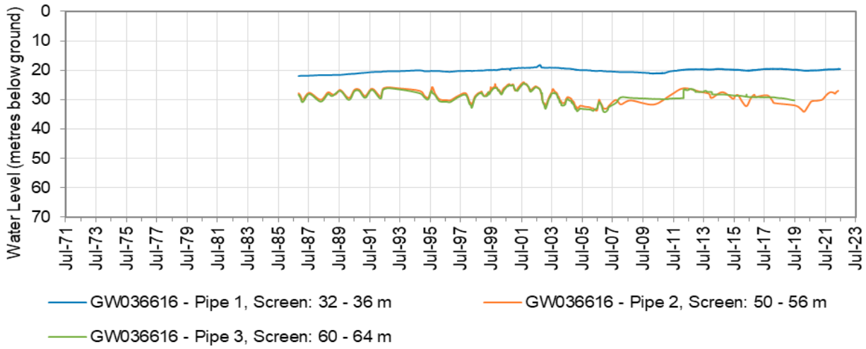
Figure 11: Hydrograph of monitoring bore GW036616 (Zone 3)
