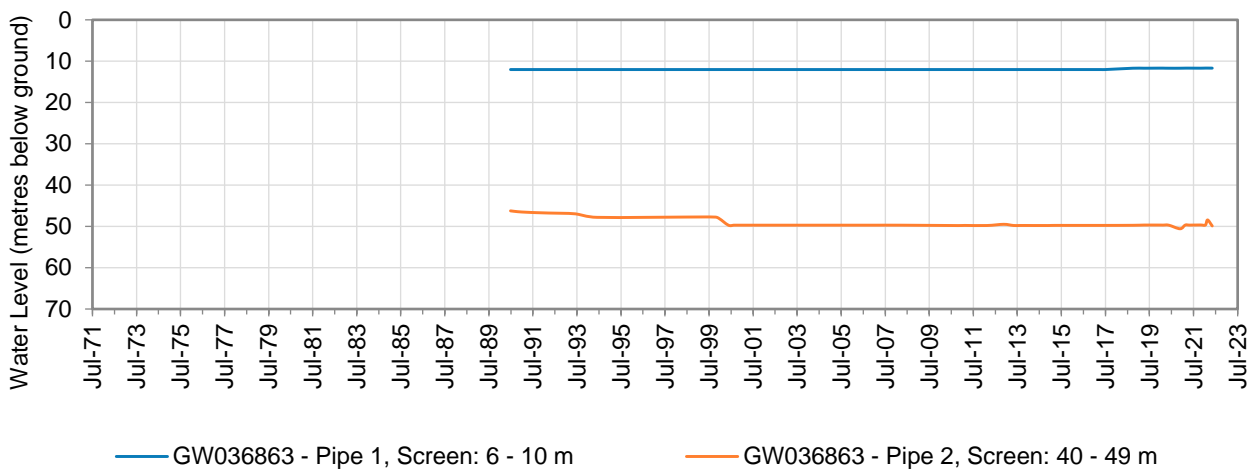
Figure 19: Hydrograph of monitoring bore GW036863 (Zone 4 / Zone 5 Boundary)
