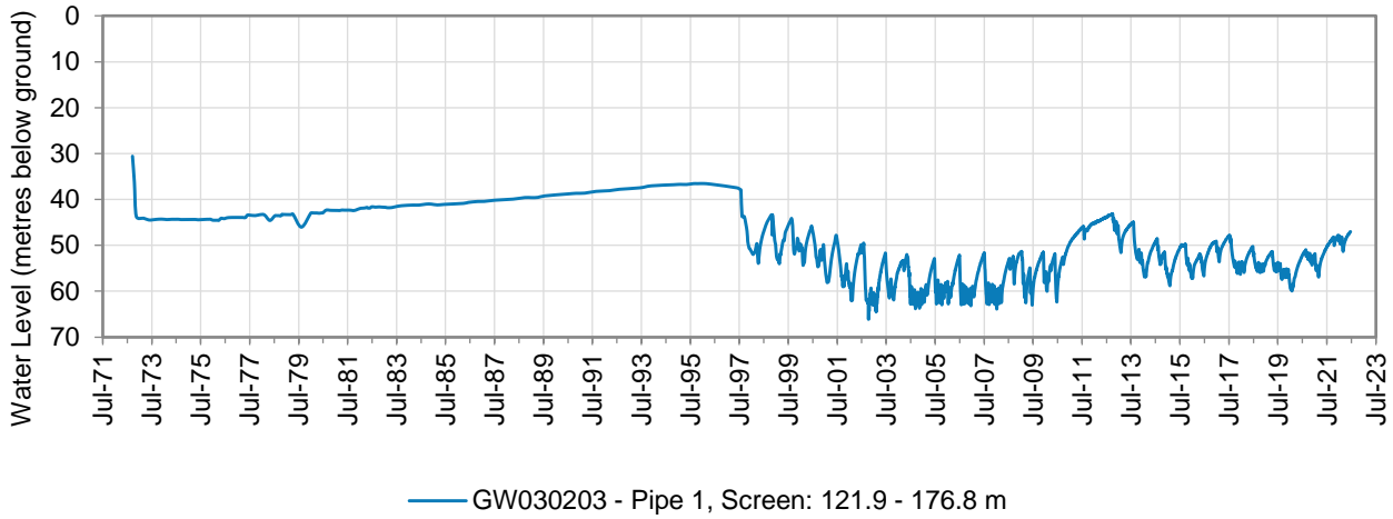
Figure 14: Hydrograph of monitoring bore GW030203 (Zone 4)
