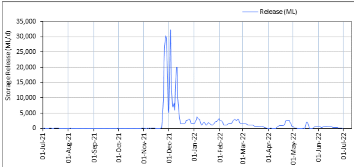
Figure 36: Copeton Dam releases
