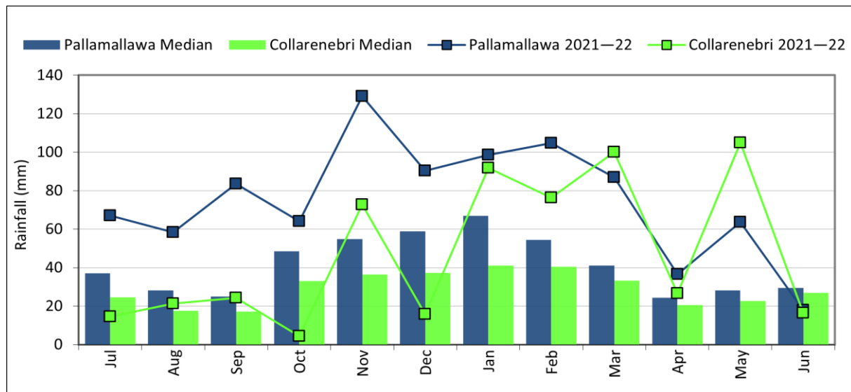
and Figure 4: Monthly rainfall deviation of the reporting period compared to historical median
