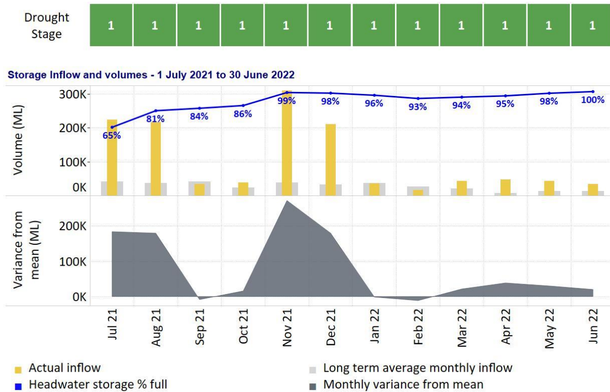
Figure 16: Drought stage for the reporting period referenced with monthly headwater storage inflows, monthly storage inflow variance from mean and storage percent full.
