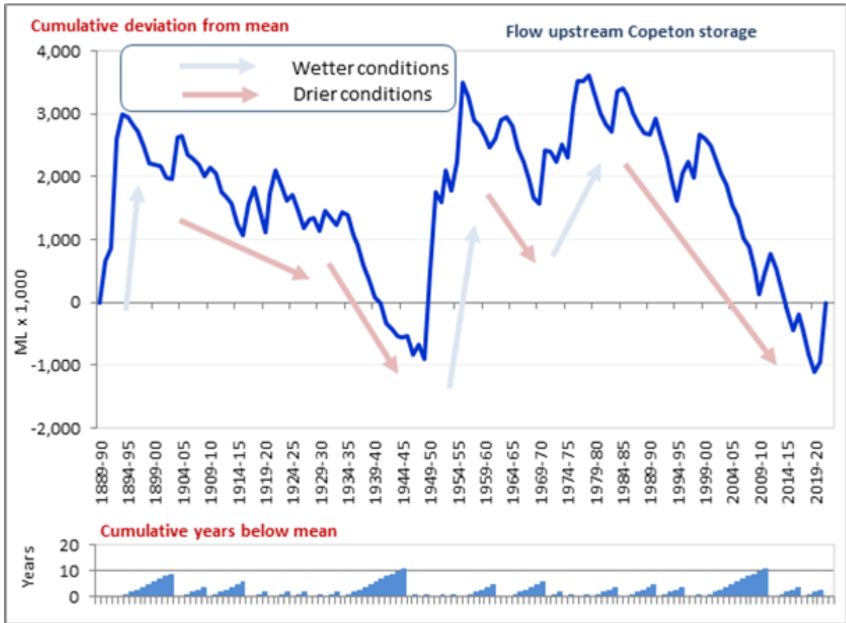
Figure 8: Long-term inflows to Copeton Dam against mean and reporting year inflow
