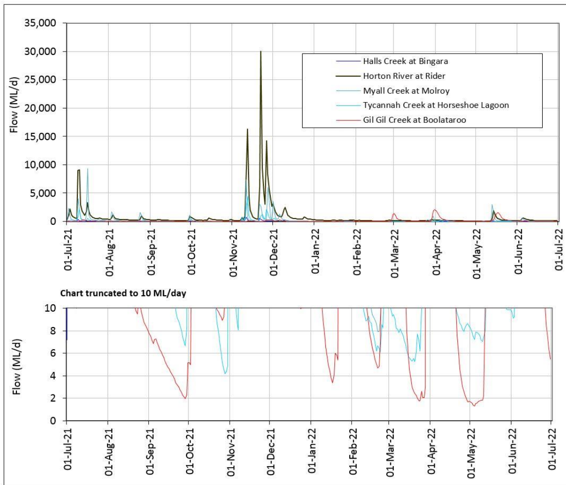
Figure 35: Gauged tributary Inflow
