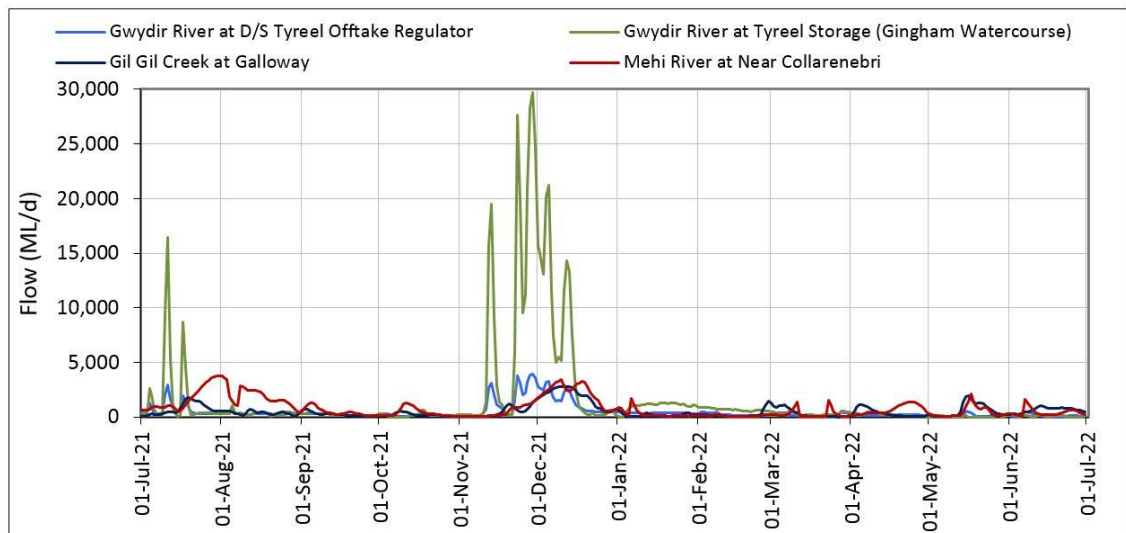
Figure 37: Gwydir end of system (includes flow to wetlands)
