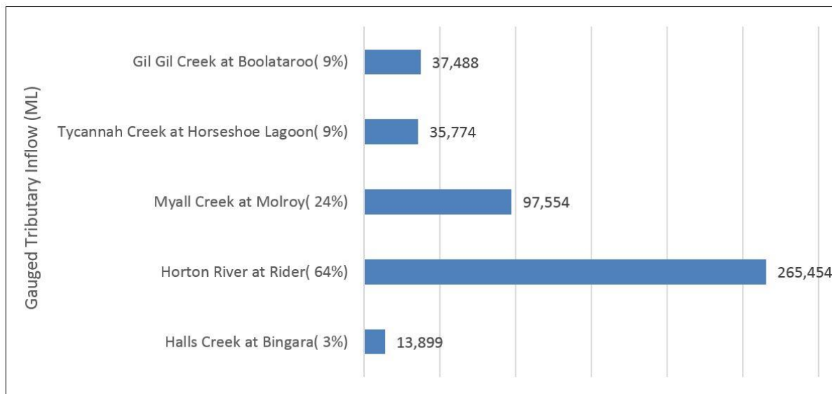
Figure 20: Measured tributary inflow contributions
