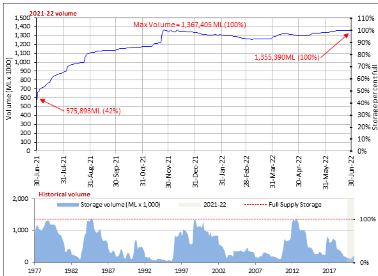
Figure 10: Copeton Dam volume and percentage of full supply volume 2021–22
