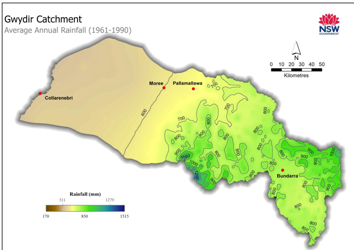
and Figure 6: Average annual rainfall in the Gwydir catchment (1961–90)
