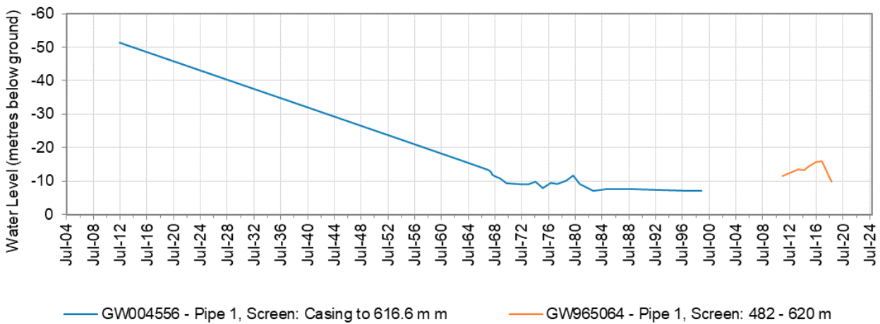
Figure 25: Hydrograph for monitoring bore GW004556 (Walgett TWS – Plugged) and GW965064 (Ulumbie No 2) – Surat Groundwater Source
