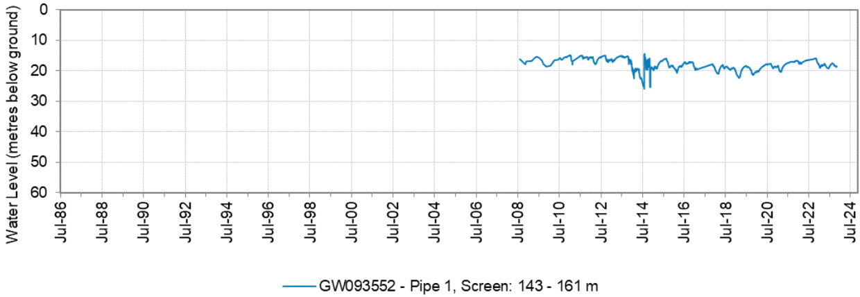
Figure 14: Hydrograph for monitoring bore GW093552 – Eastern Recharge Groundwater Source
