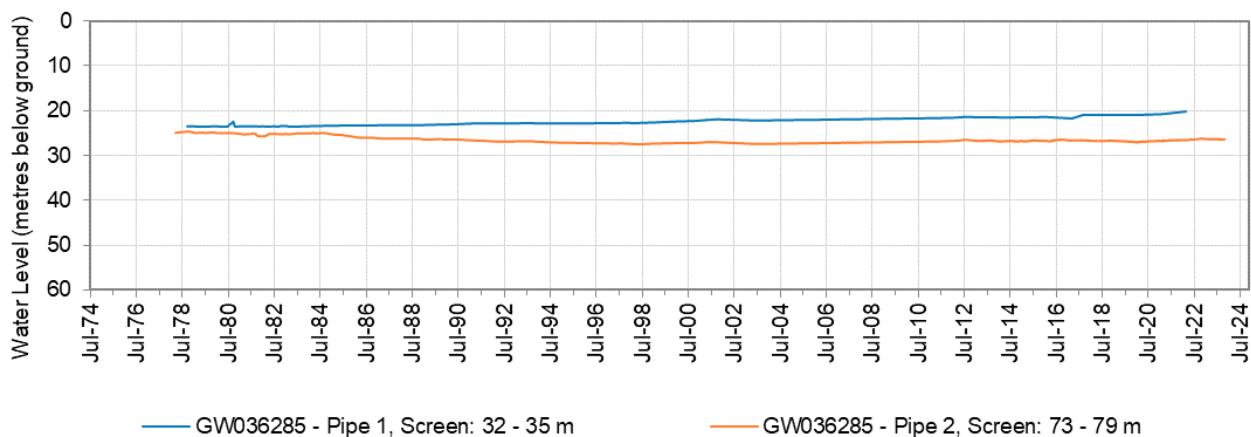
Figure 19: Hydrograph for monitoring bore GW036285 – Southern Recharge Groundwater Source
