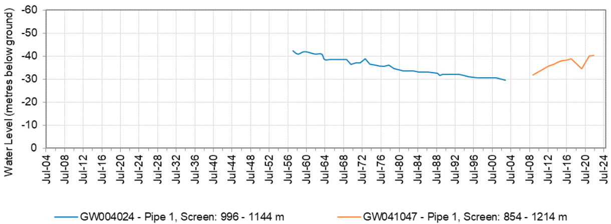
Figure 22: Hydrograph for monitoring bore GW004024 (Boomi – Plugged) and GW041047 (Boomi East No 2) – Surat Groundwater Source
