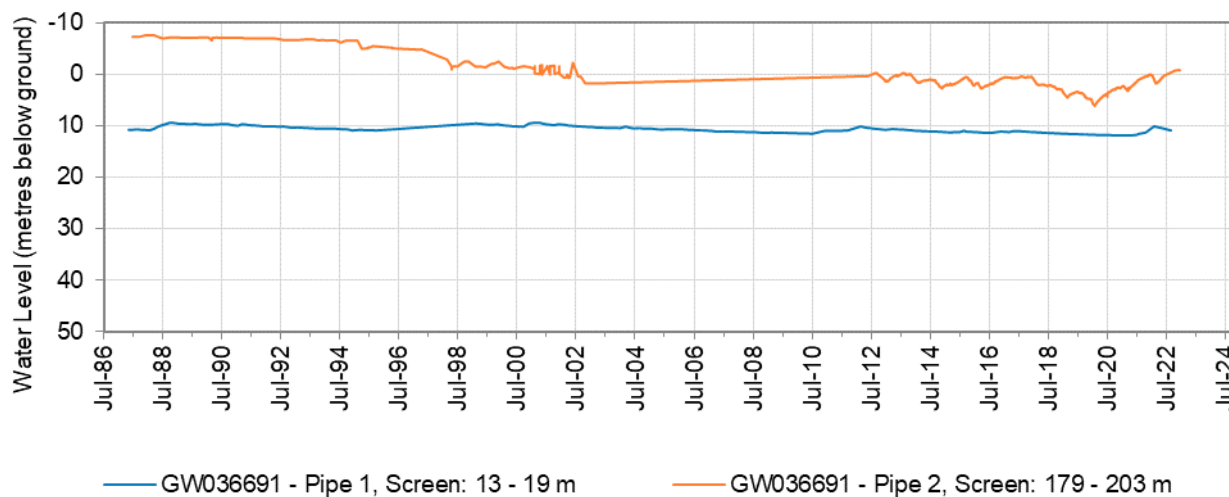
Figure 13: Hydrograph for monitoring bore GW036691 – Eastern Recharge Groundwater Source
