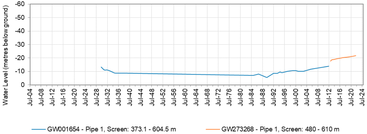
Figure 20: Hydrograph for monitoring bore GW001654 (Whittonbri – Plugged) and GW273268 (Whittonbri No 2) – Surat Groundwater Source
