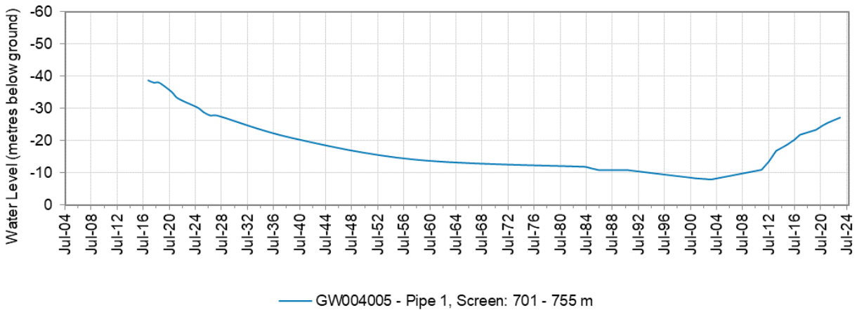
Figure 21: Hydrograph for monitoring bore GW004005 (Bangate No 2) – Surat Groundwater Source
