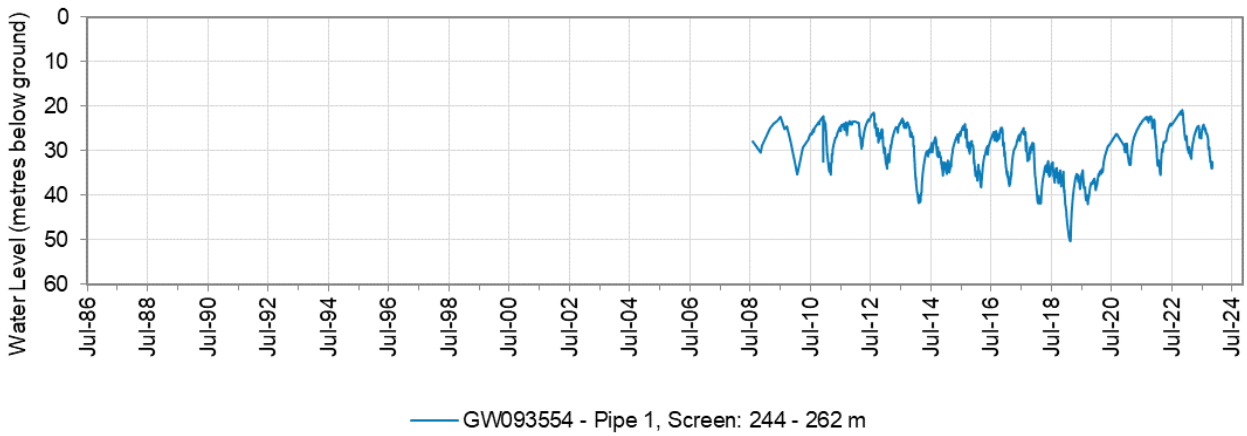
Figure 15: Hydrograph for monitoring bore GW093554 – Eastern Recharge Groundwater Source
