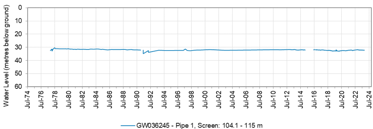
Figure 18: Hydrograph for monitoring bore GW036245 – Southern Recharge Groundwater Source
