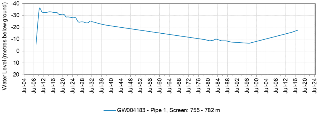
Figure 23: Hydrograph for monitoring bore GW004183 (Eulalie) – Surat Groundwater Source
