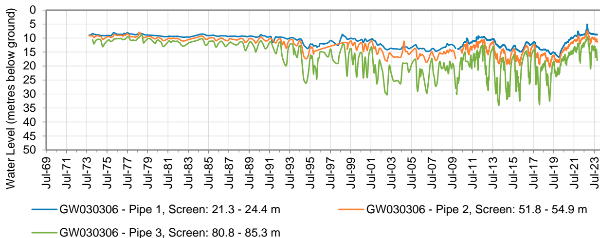
Figure 11: Hydrograph of monitoring bore GW030306
