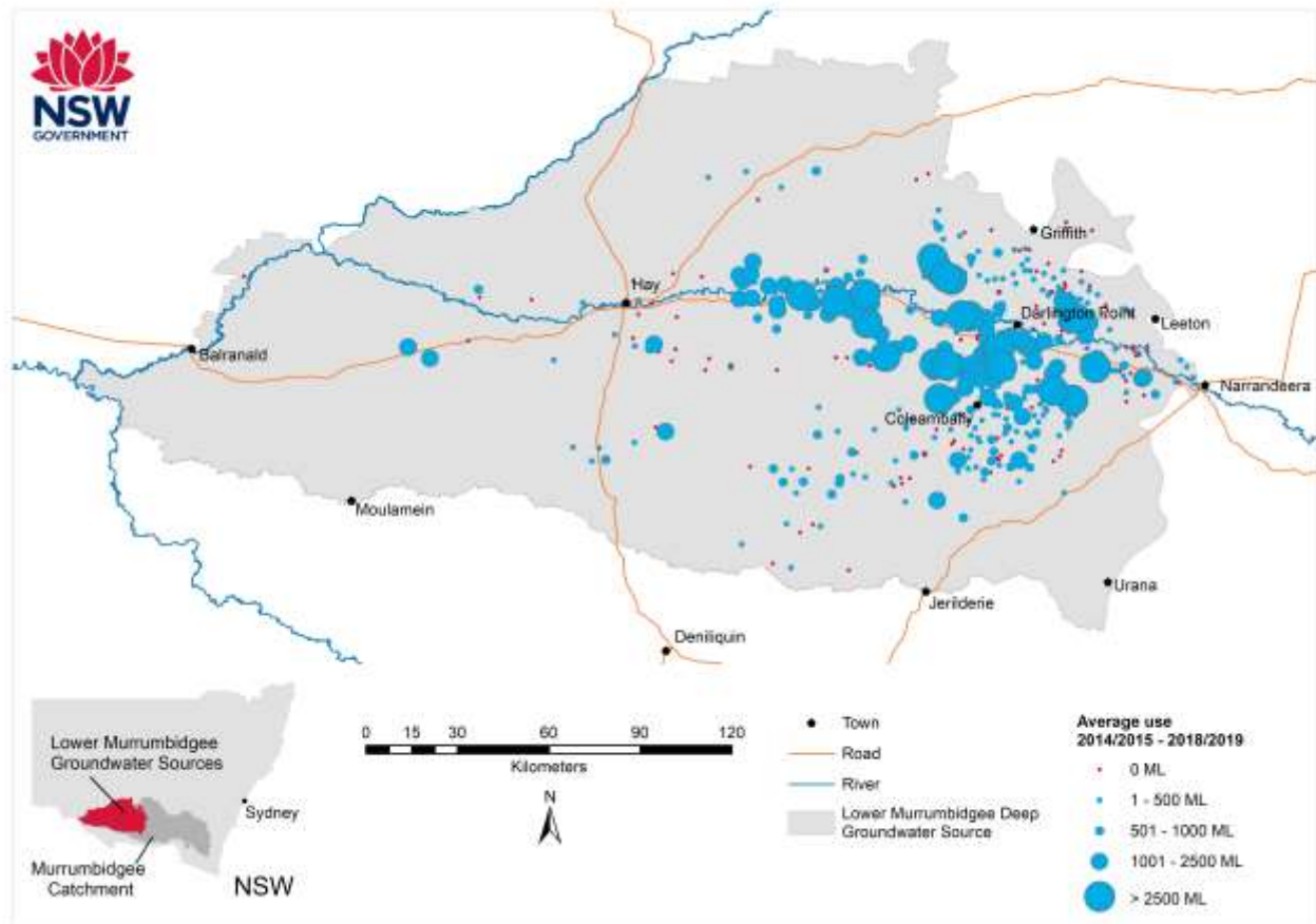
Figure 8: Lower Murrumbidgee Deep Groundwater Source water supply bores and distribution of extraction
