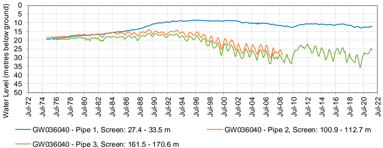
Figure 17: Hydrograph for monitoring bore GW036040
