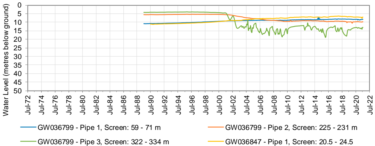
Figure 22: Hydrograph for monitoring bore GW036799
