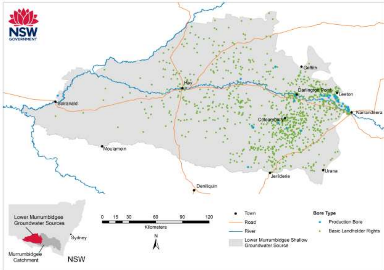
Figure 7: Lower Murrumbidgee Shallow Groundwater Source registered bores
