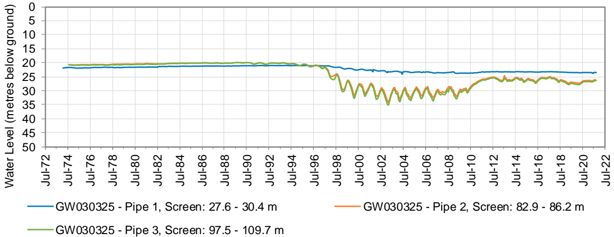
Figure 19: Hydrograph for monitoring bore GW036025
