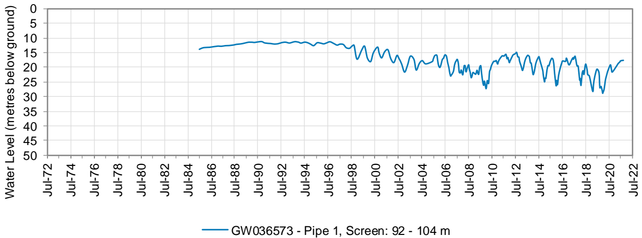
Figure 14: Hydrograph for monitoring bore GW036573
