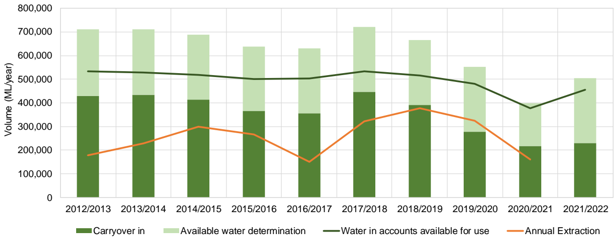
Figure 3: Account water availability and usage summary for Lower Murrumbidgee Shallow Groundwater Source
