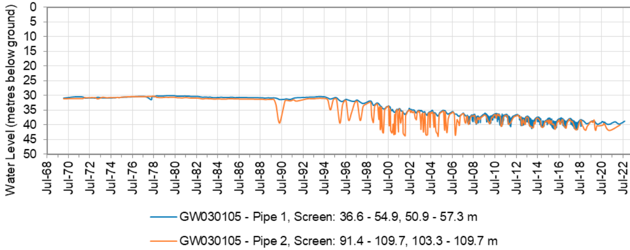
Figure 8: Hydrograph of monitoring bore GW030105
