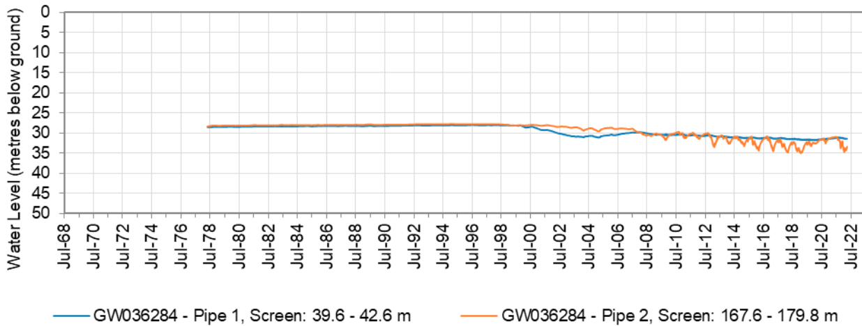
Figure 12: Hydrograph of monitoring bore GW036284
