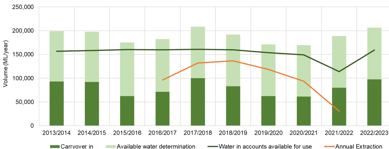
Figure 2: Account water availability and usage summary for Lower Lachlan Groundwater Source
