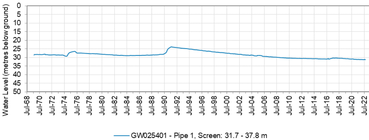
Figure 7: Hydrograph for monitoring bore GW025401
