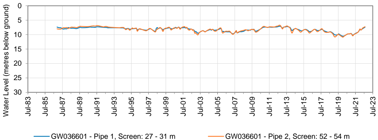
Figure 9: Hydrograph of monitoring bore GW036601
