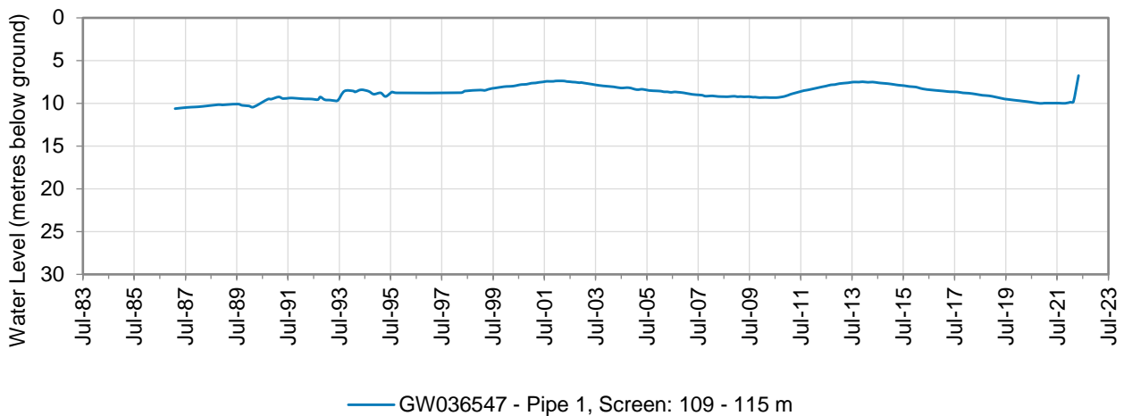
Figure 8: Hydrograph of monitoring bore GW036547
