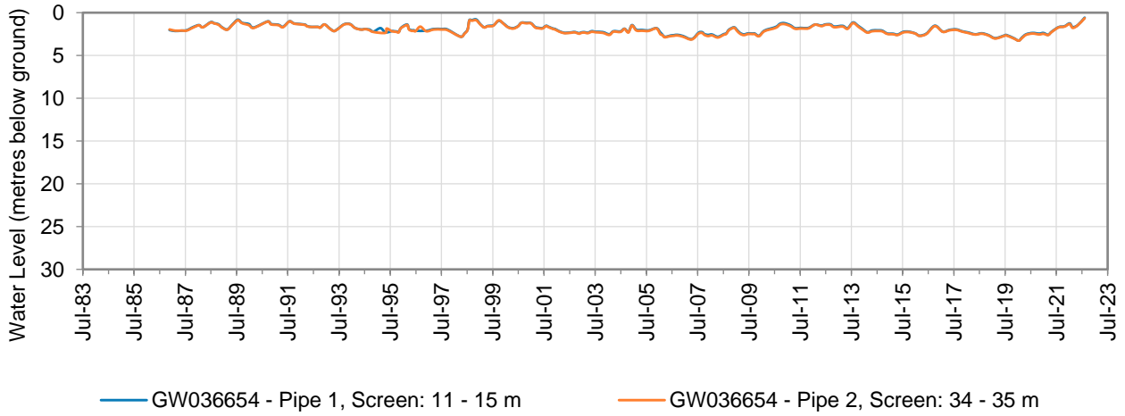
Figure 10: Hydrograph of monitoring bore GW036654
