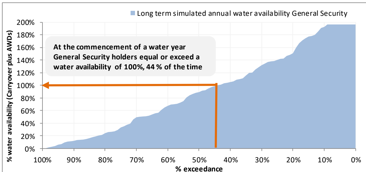
Figure 44: Start of water year simulated availability for General Security access licences (Lower Namoi)
