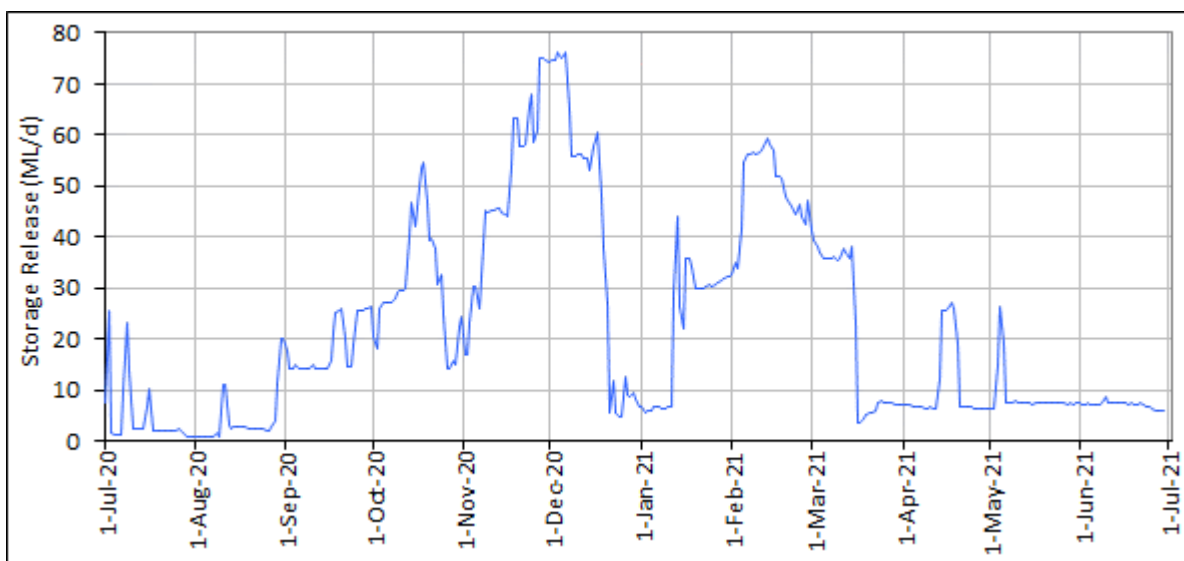
Figure 48: Split Rock Dam storages releases for reporting period
