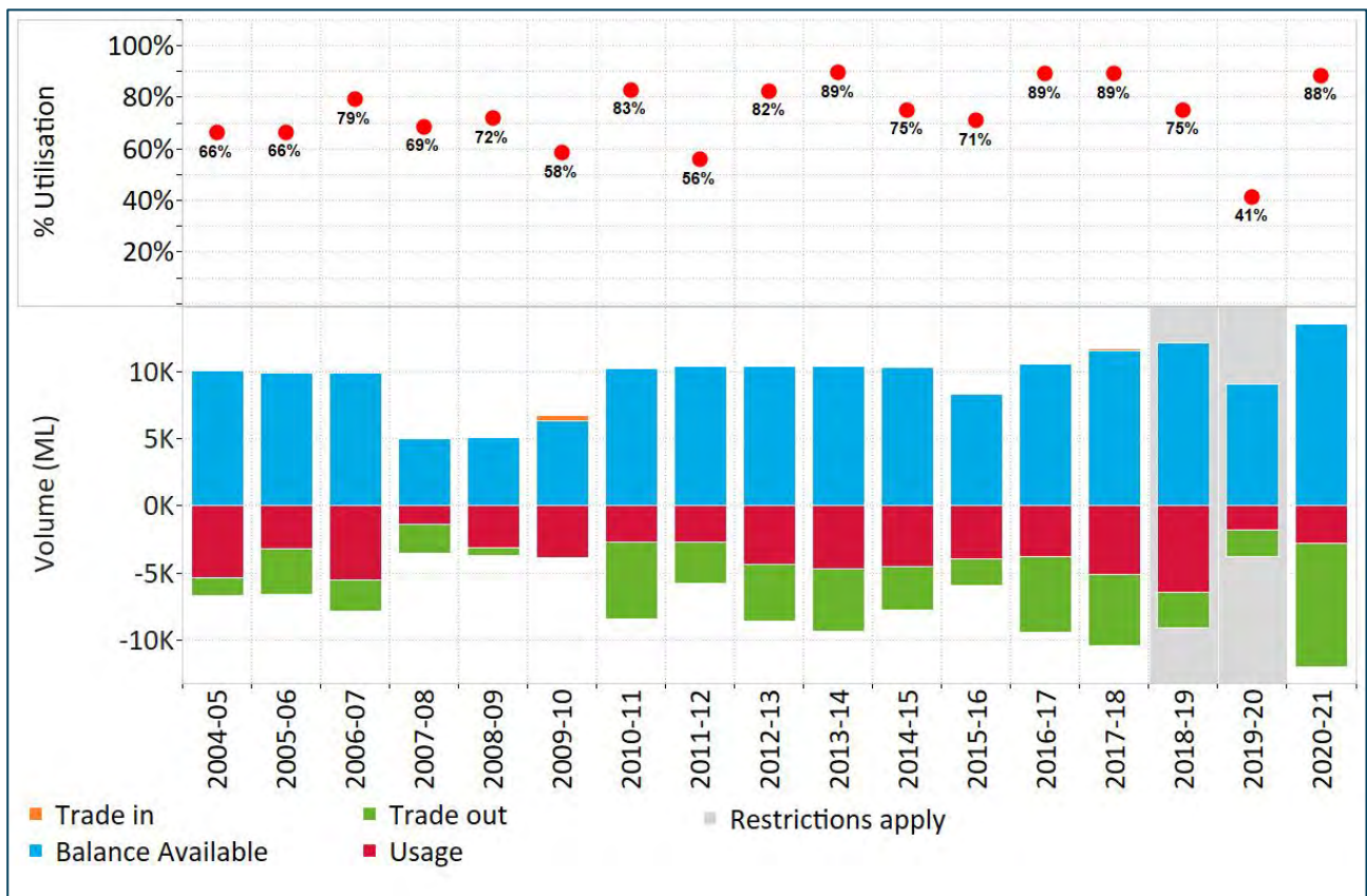
Figure 23: Upper Namoi percentage utilisation 9
