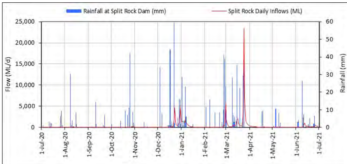
Figure 10: Daily inflows and rainfall at Split Rock 2020–21
