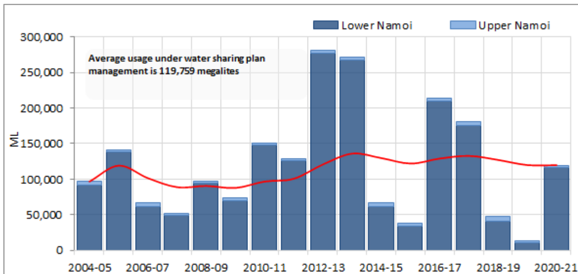
Figure 40: Namoi combined-average annual account usage and moving-average usage
