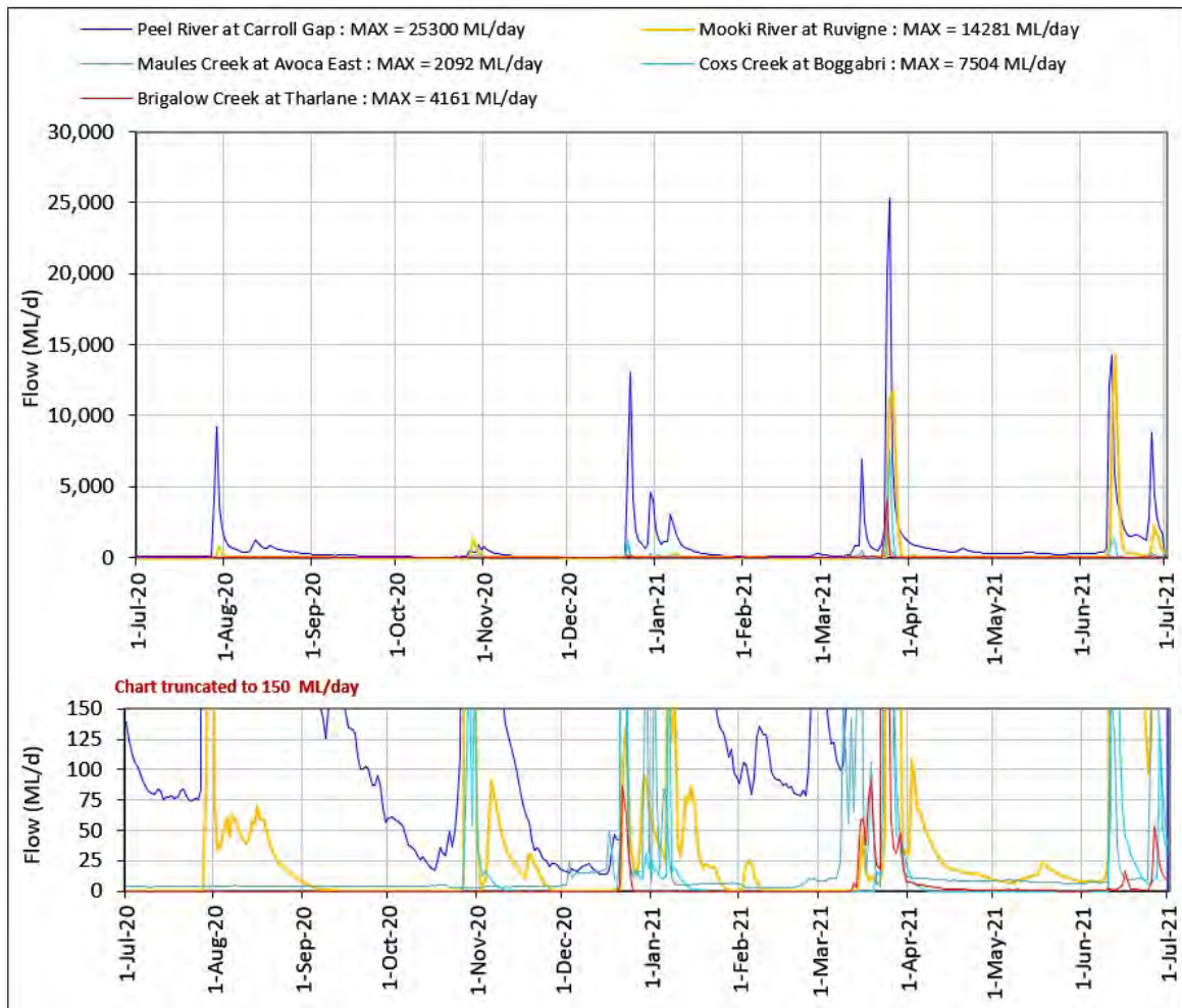
Figure 47: Lower Namoi gauged tributary inflows
