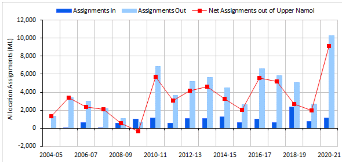
Figure 24: Upper Namoi trading summary
