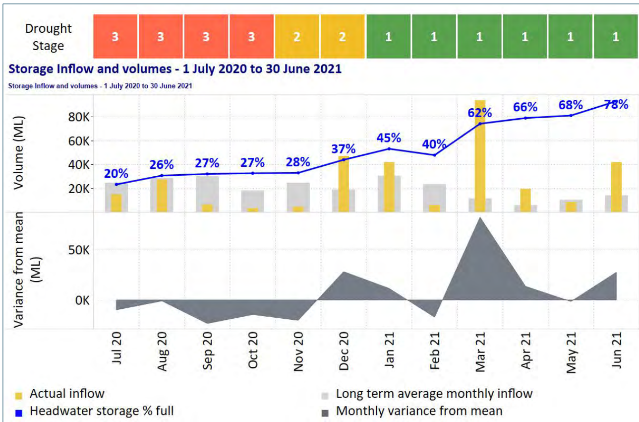
Figure 31: Drought stage for the reporting period referenced with monthly headwater storage inflows, monthly storage inflow variance from mean
