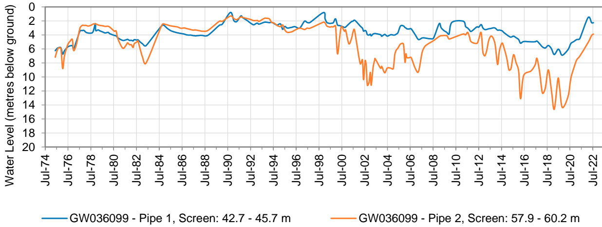
Figure 7: Hydrograph for monitoring bore GW036099
