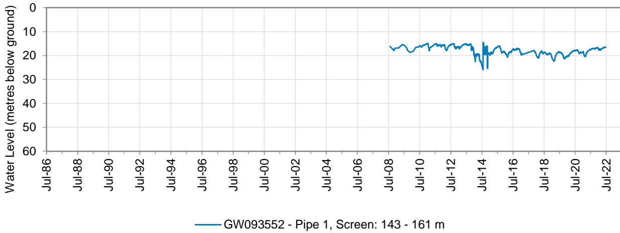
Figure 14: Hydrograph for monitoring bore GW093552 – Eastern Recharge Groundwater Source
