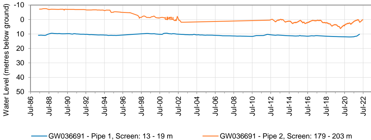
Figure 13: Hydrograph for monitoring bore GW036691 – Eastern Recharge Groundwater Source
