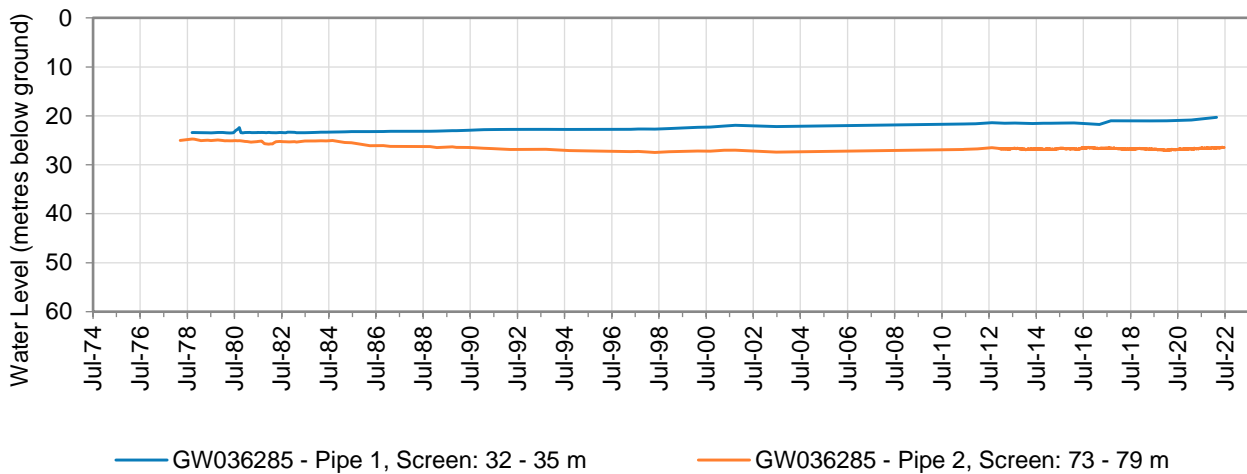
Figure 19: Hydrograph for monitoring bore GW036285 – Southern Recharge Groundwater Source
