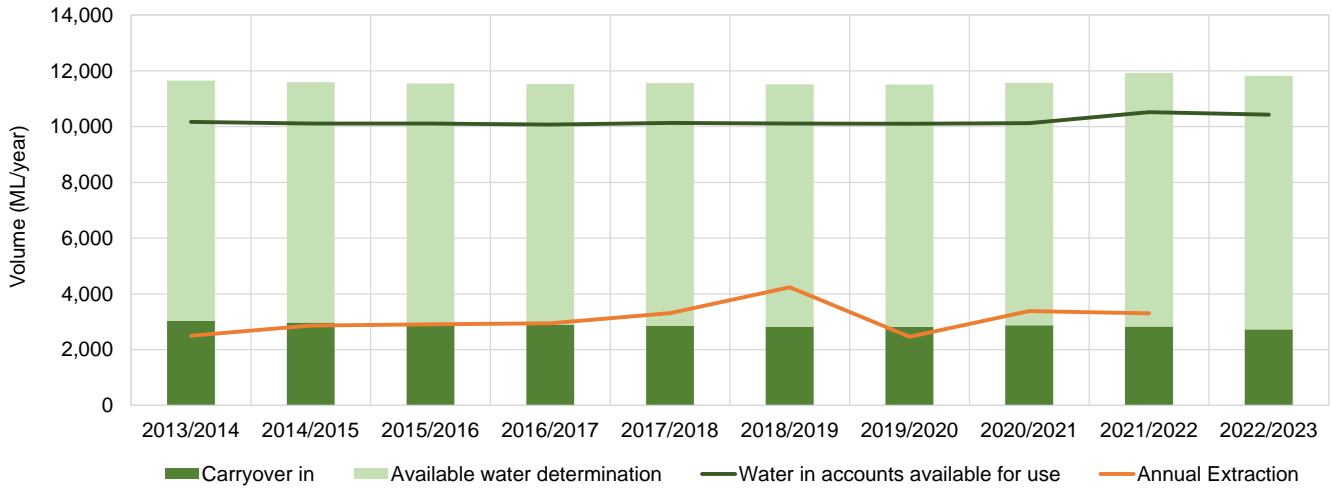
Figure 6: Account water availability and usage summary for GAB Warrego Groundwater Source
