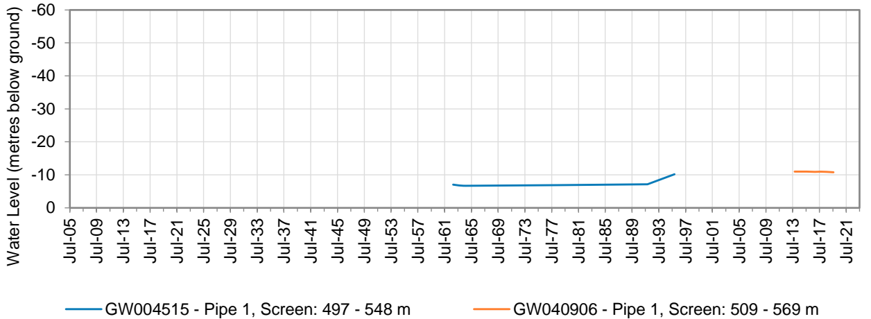
Figure 28: Hydrograph for monitoring bore GW040906 (Tineroo No 2) and GW004515 (Tineroo – Plugged) – Central Groundwater Source
