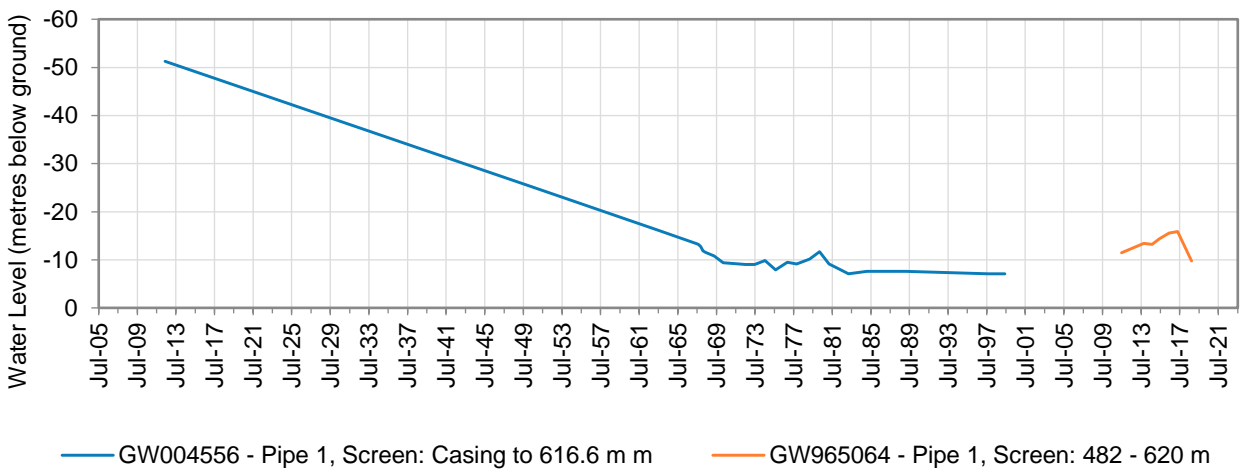
Figure 25: Hydrograph for monitoring bore GW004556 (Walgett TWS – Plugged) and GW965064 (Ulumbie No 2) – Surat Groundwater Source
