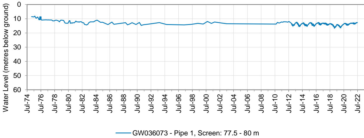
Figure 17: Hydrograph for monitoring bore GW036073 – Southern Recharge Groundwater Source
