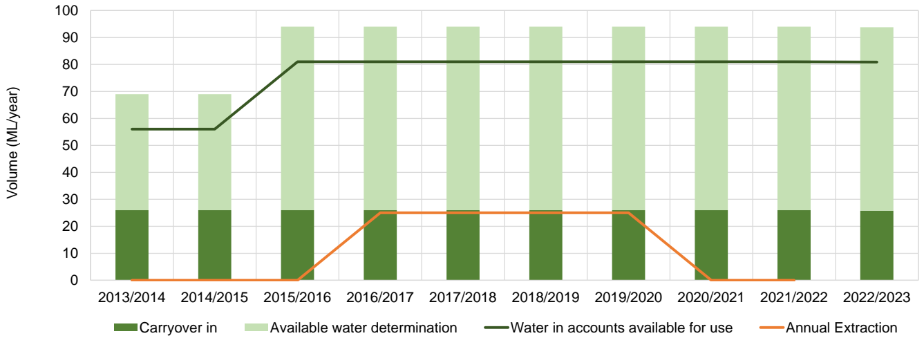
Figure 3: Account water availability and usage summary for GAB Eastern Recharge Groundwater Source
