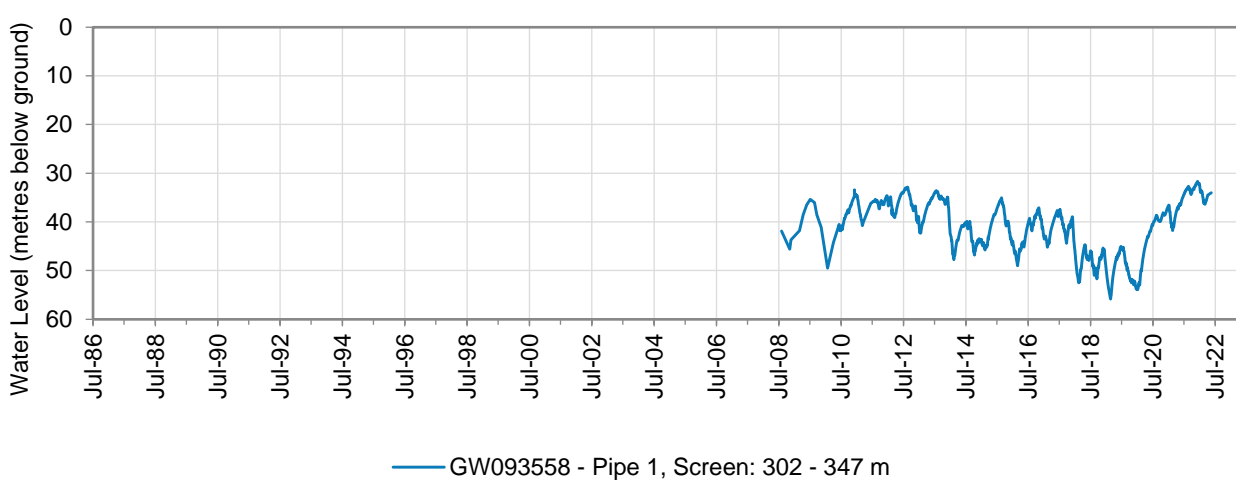
Figure 16: Hydrograph for monitoring bore GW093558 – Eastern Recharge Groundwater Source
