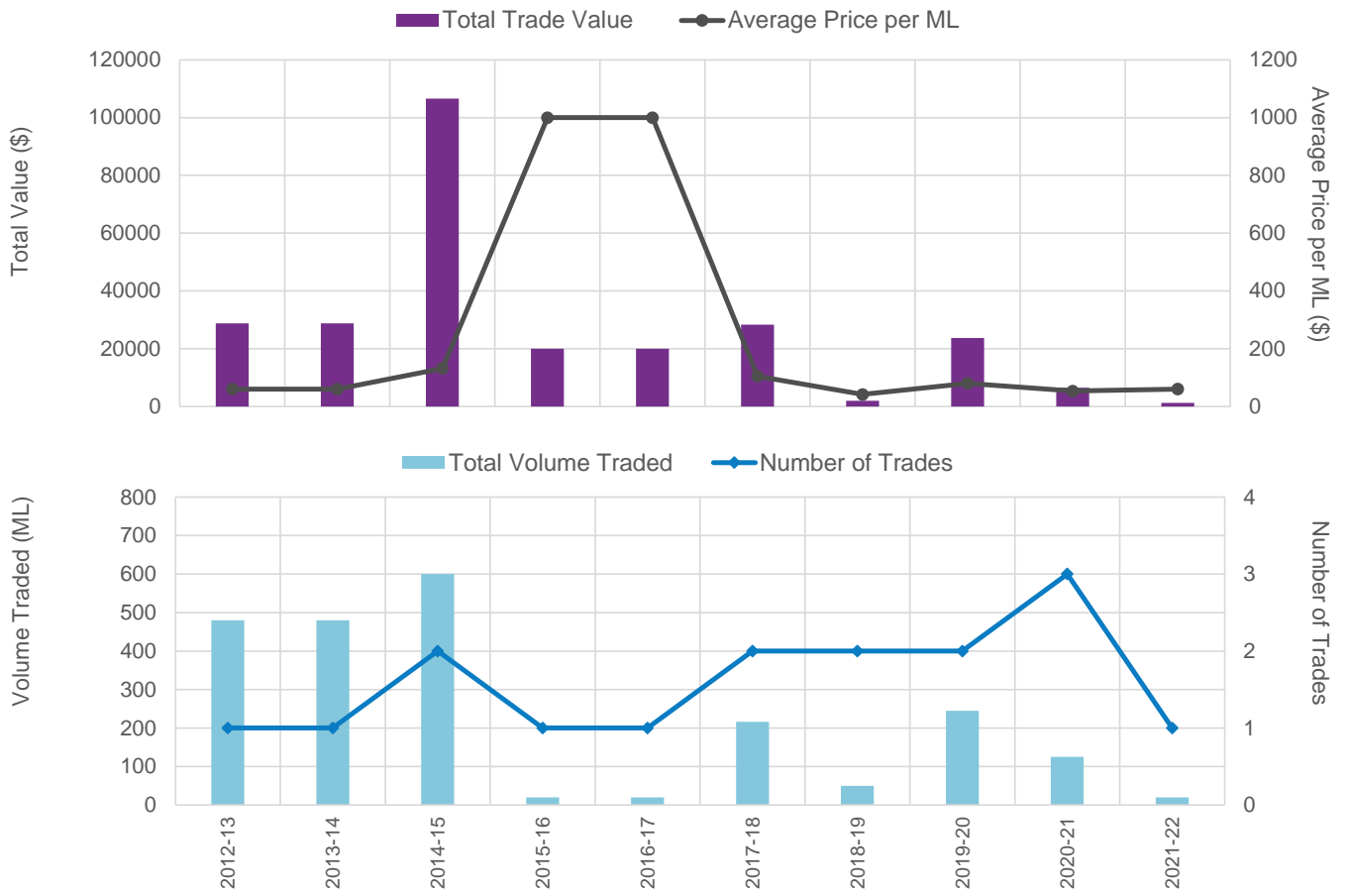
Figure 8: Southern Recharge Groundwater Source temporary trade statistics
