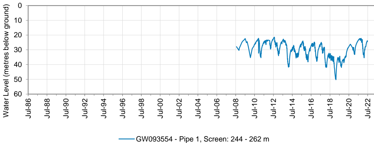
Figure 15: Hydrograph for monitoring bore GW093554 – Eastern Recharge Groundwater Source
