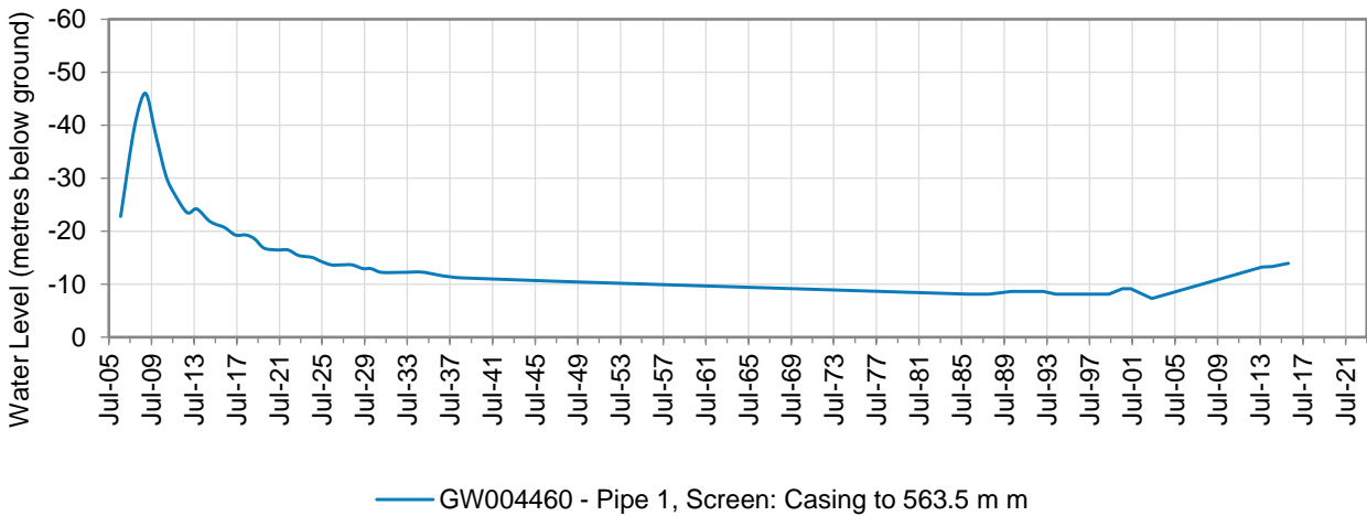
Figure 24: Hydrograph for monitoring bore GW004460 (Roma) – Surat Groundwater Source
