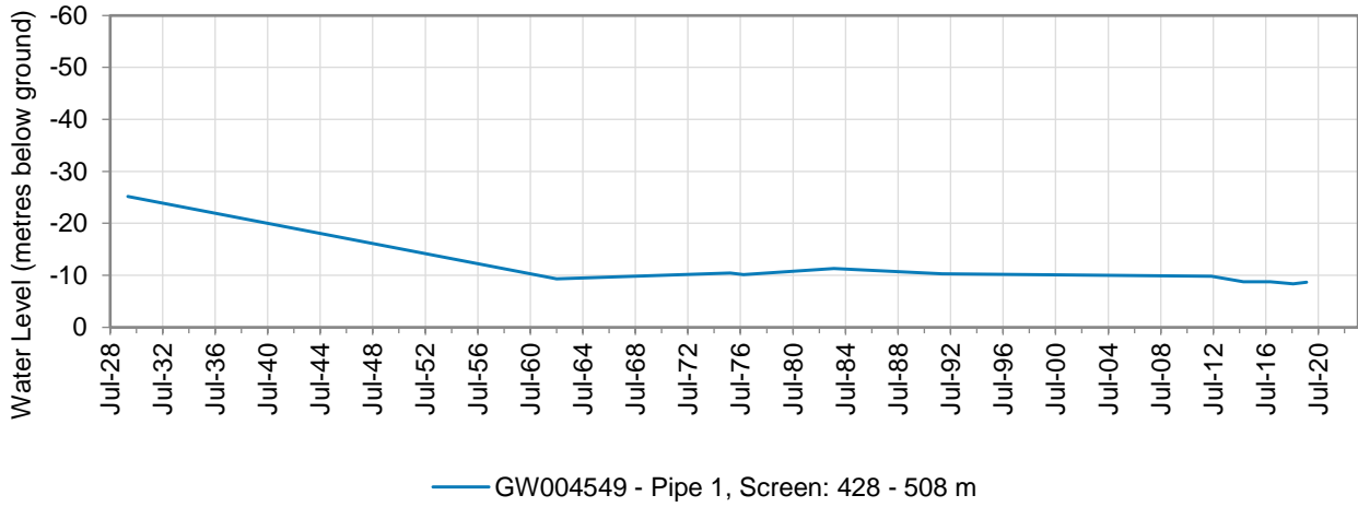
Figure 29: Hydrograph for monitoring bore GW004549 (Urisino No 4) - Central Groundwater Source
