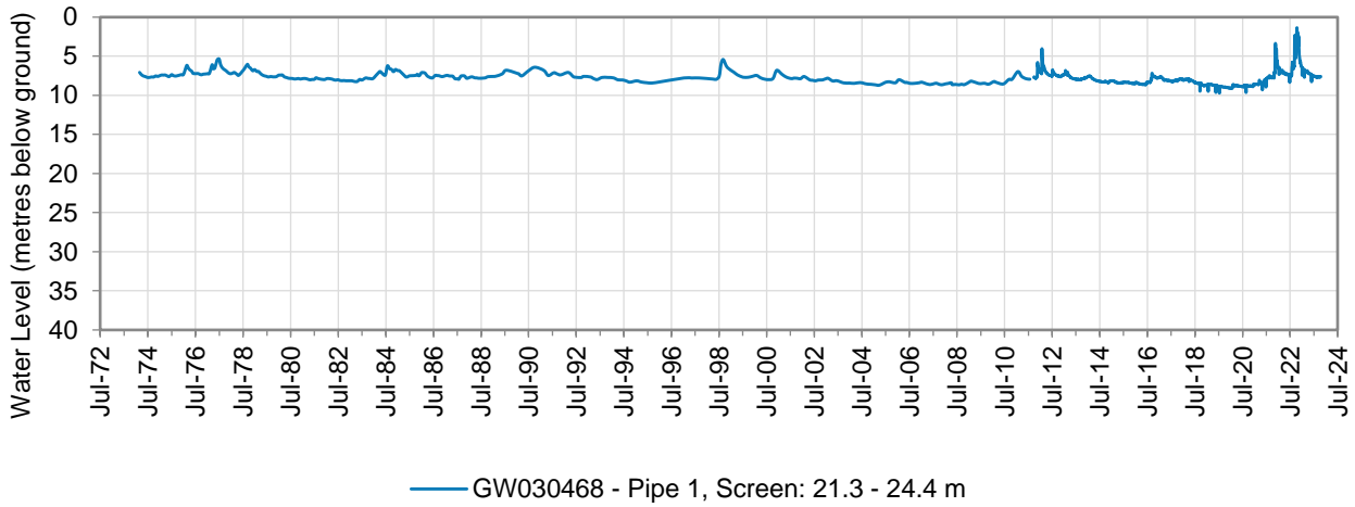
Figure 12: Hydrograph of monitoring bore GW030468 – Upper Namoi Zone 4 Groundwater Source
