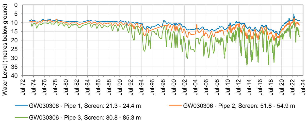
Figure 8: Hydrograph for monitoring bore GW030306 – Upper Namoi Zone 4 Groundwater Source
