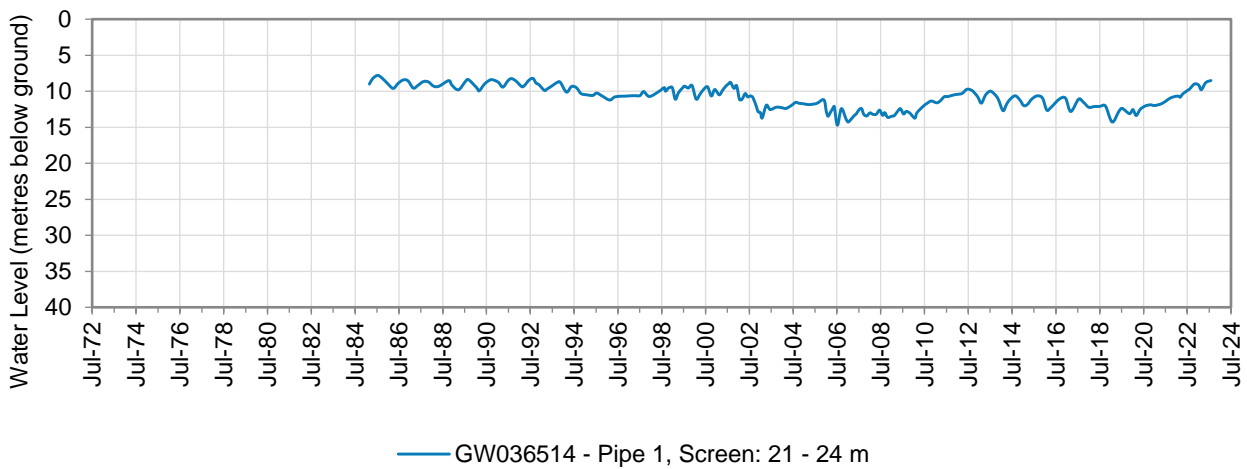
Figure 11: Hydrograph of monitoring bore GW036514 – Upper Namoi Zone 4 Groundwater Source
