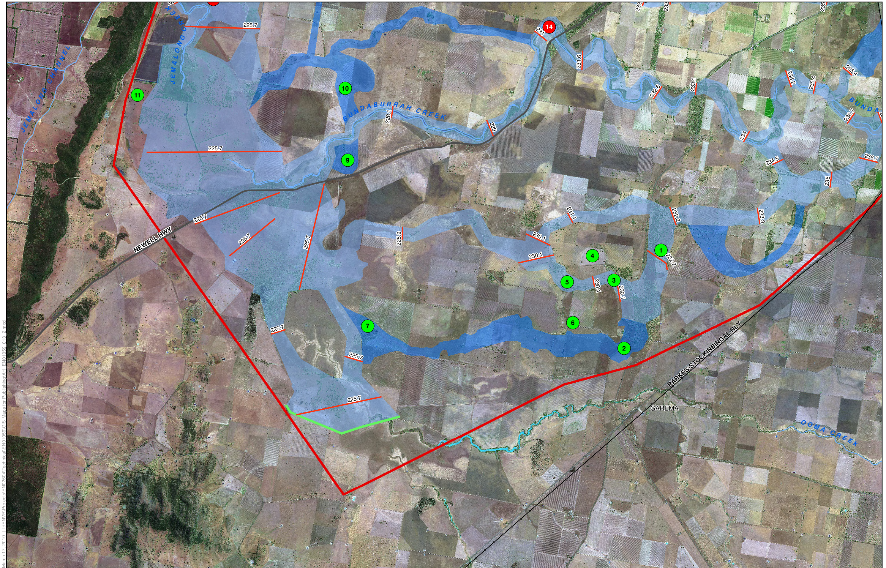
Figure 2 Lachlan River Gooloogong to Jemalong Gap Floodplain Management-Plan Floodway Network Sheet 2 of 4
